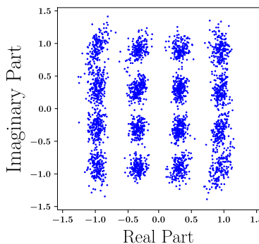
(f) Transmitter IQ imbalance compensation
