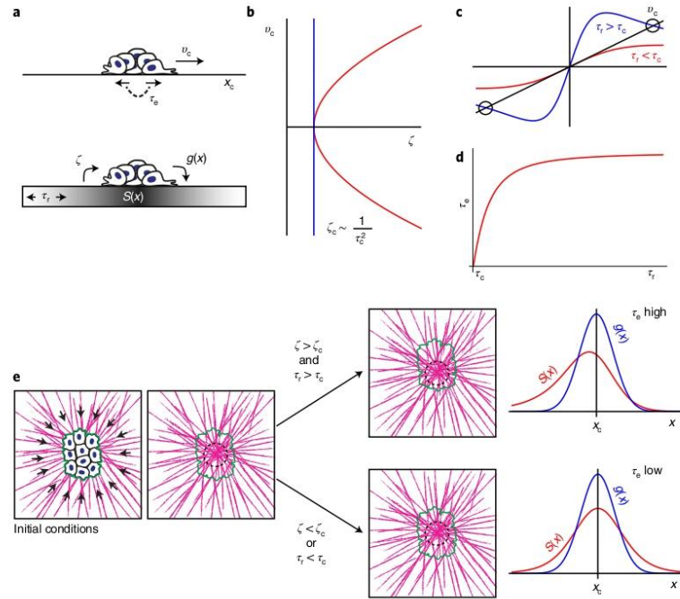
Fig. 3 | Theoretical model of persistent migration on a viscoelastic substrate. a , Schematic description of the model. A cluster of cells moves along the axis x_c with velocity v_c . The probability of switching migration direction is given by the timescale \tau_e . The cell cluster interacts with the substrate according to a symmetric forcing function g(x) , resulting in a deformation of the substrate given by S(x) . The deformation in the substrate leads to a change in the activity in the cell cluster via the coupling \zeta . As the substrate is viscoelastic, the relaxation is characterized by the timescale \tau_r . b , The cell migration velocity v_c undergoes a supercritical pitchfork bifurcation at \zeta = \zeta_c . Here, v_c is plotted as a function of \zeta for g(\xi') = e^{-\xi'^2/2} (Supplementary Note 1). c , Solutions for migration velocity v_c for substrate relaxation times above or below the critical relaxation time. Solutions are shown by the intersection with the black line. While for \tau_r < \tau_c , only a stable ( v_c = 0 ) solution exists, a positive solution for v_c exists for \tau_r > \tau_c . d , Cluster persistence timescale \tau_e as a function of the substrate relaxation timescale \tau_r relative to the critical relaxation time \tau_c . e , Interpretation of the model as it relates to experiments. Initially symmetric inward-directed tractions (left arrows) generate radially oriented collagen fibres (magenta), with a high collagen density in the centre of the cluster. After symmetry breaking, for networks with sufficient cell–substrate coupling ( \zeta > \zeta_c ) and relaxation time ( \tau_r > \tau_c ), clusters are predicted to migrate persistently (that is, \tau_e is high) due to the offset between the driving function g(x) and the substrate deformation S(x) (top). If the coupling or relaxation times are below the critical values, g(x) and S(x) are both symmetric around x_c and low persistence migration (low \tau_e ) is predicted (bottom). Green contours, cell cluster position; black dotted circles, collagen centre of mass.
