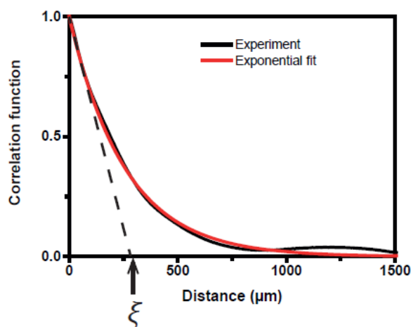
Figure 18. Extraction of the correlation length \xi from the spatial autocorrelation of the orientation map \theta .
