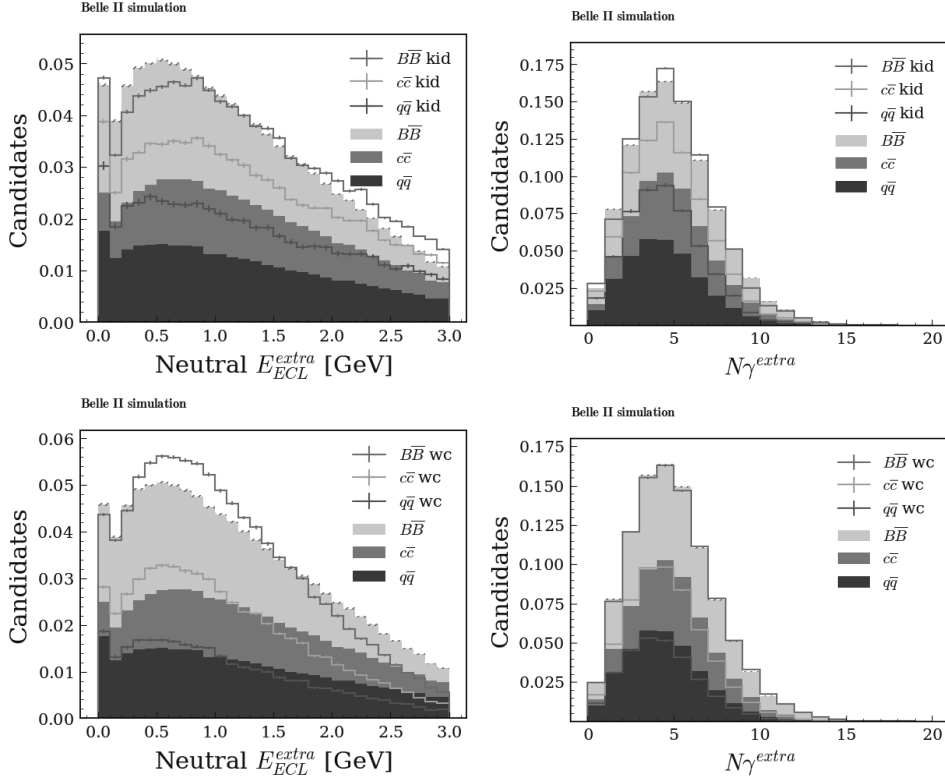
Figure 5.21: Distribution of the neutral ECL extra energy (left) and N_{\gamma} (right) for the particle ID (top, line histograms) and wrong B -meson charge (bottom, line histograms) sidebands. The filled histograms show the relevant distributions for the simulated background samples passing the signal selection, before the BDT output cut. The dashed histograms correspond to the statistical uncertainty on the total simulated sample.
