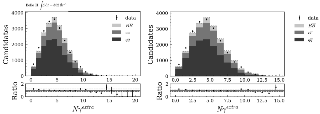
Figure 5.22: Distribution of the photon multiplicity N_{\gamma} for the right B -meson charge subsample of the particle ID sideband before (left) and after (right) correction. Distributions are shown for simulated background events (filled) and data (points).
