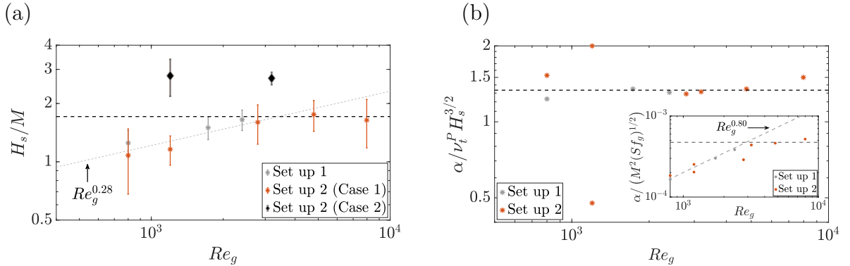
FIGURE 4.10 – (a) Evolution of H_s , the depth over which the eddy viscosity is almost constant, as a function of the grid Reynolds number, Re_g . Here H_s is expressed as the distance under the grid. (b) Evolution of \alpha , the proportionality constant of \nu_t^S when z > H_s , as a function of the Reynolds number.
