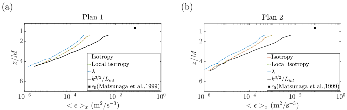
Figure S33 – Vertical profiles of the dissipation rate, \epsilon , calculated from four definitions with different assumptions. They was obtained in two laser sheets at (a) x = L/4 and (b) x = L/2 from the border of the tank.
