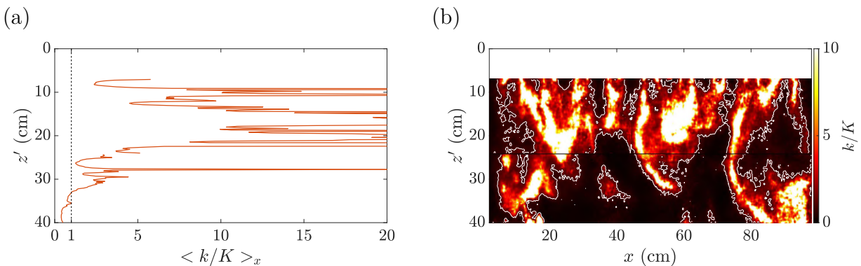
FIGURE 4.4 – Example at Re_g = 800 of : (a) Depth profile of the turbulent kinetic energy, k , over the kinetic energy based on the mean flow, K . (b) Map of k/K to ensure that the turbulence is homogeneous. The white contour line represents k = K .
