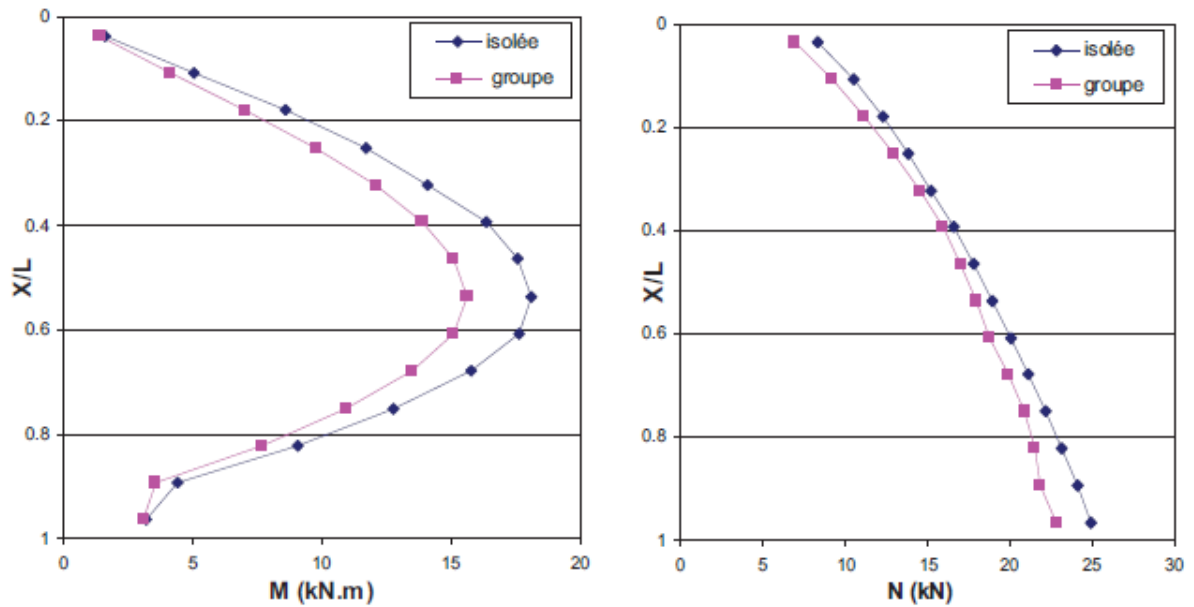
Figure 2.16: internal forces comparison in single inclusion and a group of 2x2 inclusions (Hatem, 2009)
