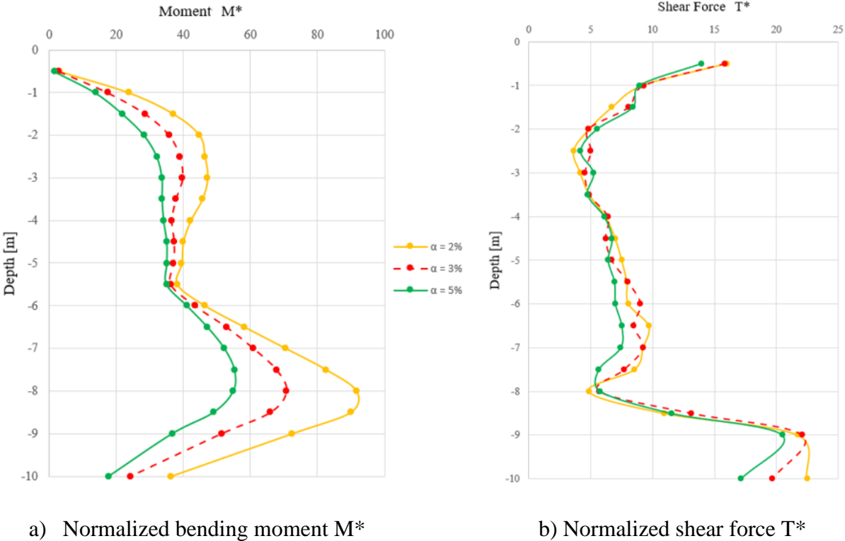
Figure 4.13: Influence of the cover ratio on the response of rigid inclusion: a) Normalized bending moment, b) Normalized shear force. [ M^* = M / \rho D^4 a_g ], [ T^* = T / \rho D^3 a_g ]
