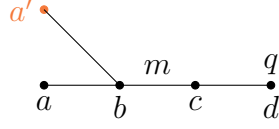
Figure 3.3: The graph \Omega_{m,q} build out of the Dyer graph \Gamma_{m,q} for some m, q \in \mathbb{N}_{\geq 2} . There are two types of vertices: V \subset V(\Lambda_{m,q}) and \{v' \mid v \in V_{\infty}\} . Every vertex and every edge is labeled by 2 if not specified otherwise.
