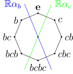
Figure 2.1: The Coxeter polytope of (\langle\langle b, c \mid b^2 = c^2 = (bc)^4 = \mathbf{e} \rangle\rangle, \{b, c\})
