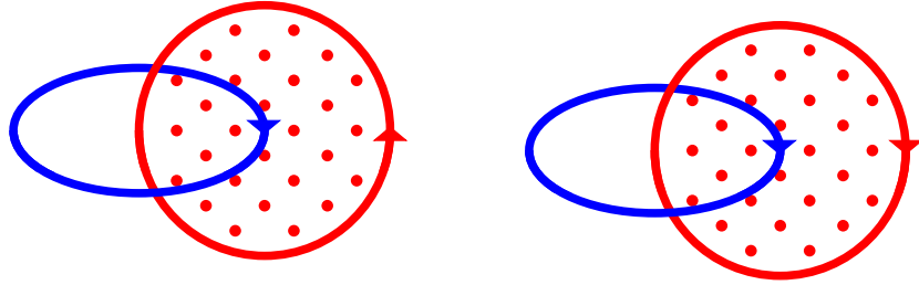
(a) The red (dotted) Seifert surface is oriented in a trigonometric (a.k.a. counterclockwise) manner.
