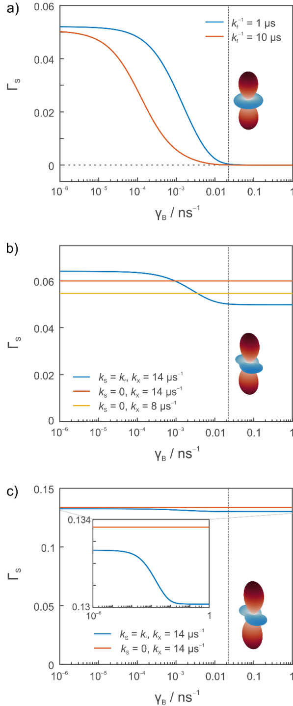
Figure 2.3: Directional magnetic field effects of radical pair and triad systems of topology \text{FADH}^*/\text{O}_2^{\bullet-} or \text{FADH}^*/\text{O}_2^{\bullet-}/\text{Y}^* subject to random-field spin relaxation in \text{O}_2^{\bullet-} . a) \text{FADH}^*/\text{O}_2^{\bullet-} for k_f^{-1} = 1 \mu\text{s} and 10 \mu\text{s} , k_S = k_f and k_T = 0 ; b) and c) \text{FADH}^*/\text{O}_2^{\bullet-}/\text{Y}^* for k_f^{-1} = 1 \mu\text{s} and 10 \mu\text{s} , respectively, different k_S and k_X as indicated in the legends, and k_T = 0 . The \text{Y}^* has been modelled after Y319 in DmCry . For the three-radical systems, the hyperfine interaction of N5, N10 and H5 in \text{FADH}^* and of the two ortho-protons in \text{Y}^* have been considered; a) additionally included H \beta 1 and H6 in \text{FADH}^* . The inserts on the right illustrate the anisotropy of the yield of the signalling state evaluated for \gamma_B = 0.022 \text{ ns}^{-1} , the relaxation rate expected for a viscous cellular environment, and the conditions represented by the blue lines. These diagrams are not drawn to scale.
