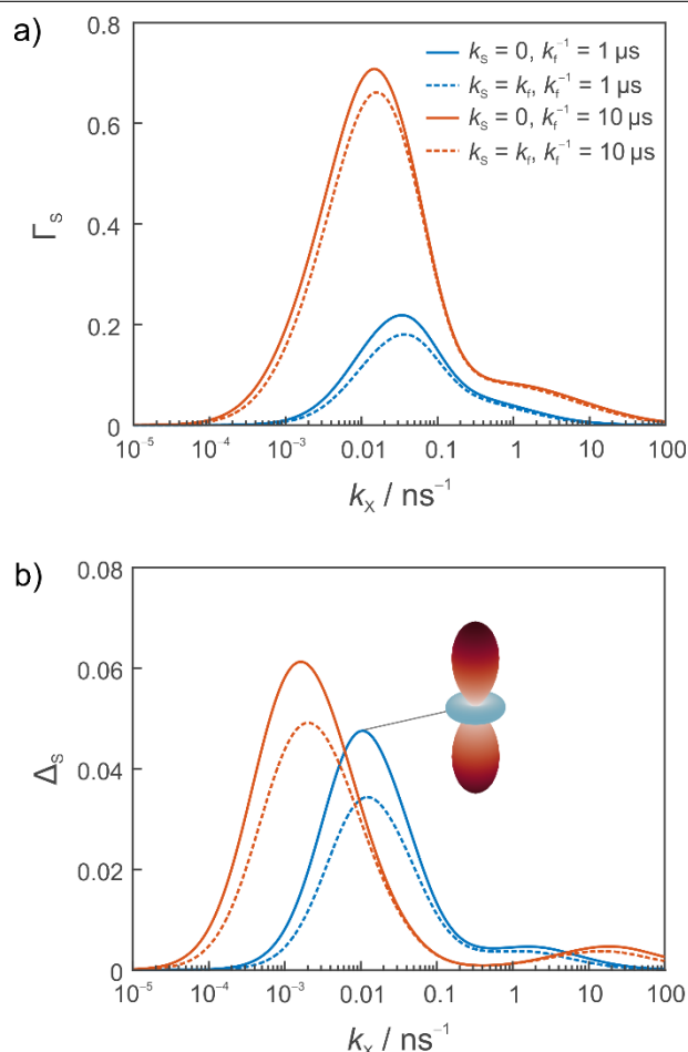
Figure 2.6: Directional magnetic field effects evaluated for \text{FADH}^{\bullet}/\text{O}_2^{\bullet-}/\text{Asc}^{\bullet-} radical triad, where \text{Asc}^{\bullet-} denotes a freely diffusing ascorbyl radical. The relative anisotropy (a) and absolute spread of the reaction yield of the signalling state are shown in a) and b), respectively. k_f and k_S are indicated in the legend of a), which applies throughout. The simulations have included the hyperfine interactions of N5, N10, H5, H6, H \beta 1 in \text{FADH}^{\bullet} and the isotropic interaction of H4 in \text{Asc}^{\bullet-} . The model does not depend on the identity of the cryptochrome.
