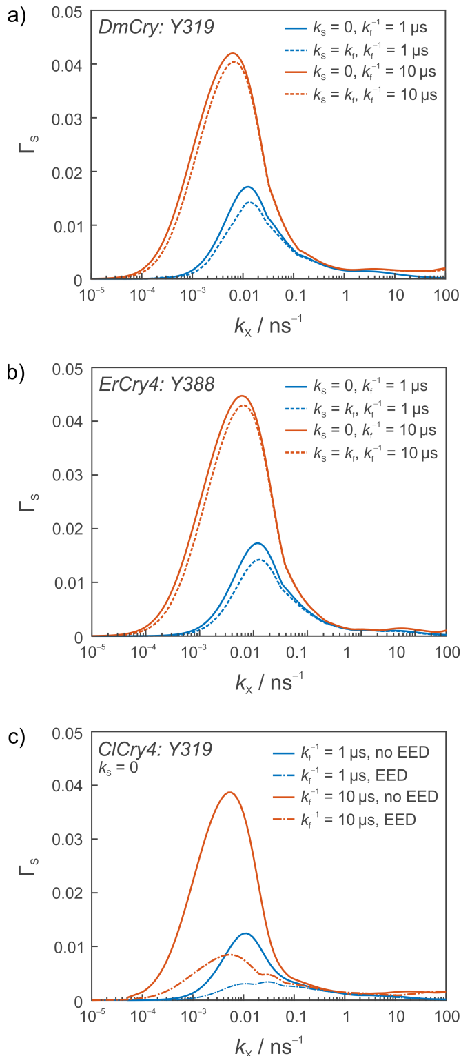
Figure 2.4: Directional magnetic field effects evaluated for models of \text{FADH}^*/\text{O}_2^{\bullet-}/\text{Y}^* in the limit of infinitely fast spin relaxation in \text{O}_2^{\bullet-} presented as a function of the scavenging rate constants k_x . The scavenger radical \text{Y}^* has been identified with a) Y319 in DmCry , b) Y388 in ErCry4 , and c) Y319 in ClCry4 , respectively. k_s and k_f are specified in the legends; k_T = 0 . All simulations included the hyperfine interactions of N5, N10, H5, H6, H \beta 1 in \text{FADH}^* and Ho1, Ho2, and H \beta 2 in \text{Y}^* . For a) and b), EED interactions have been neglected; c) provides simulations with (dashed-dotted lines) and without (solid lines) EED interactions.
