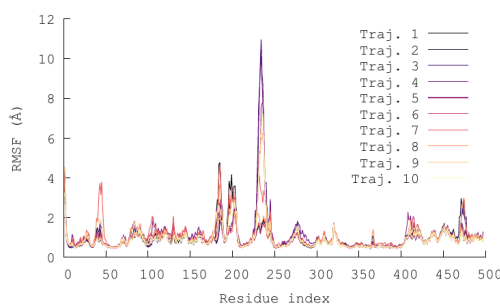
(c) Cl^-
