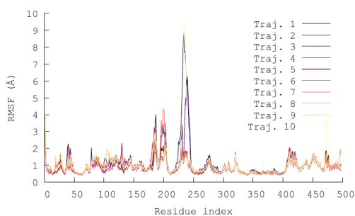
(b) O_2^{\bullet-}
