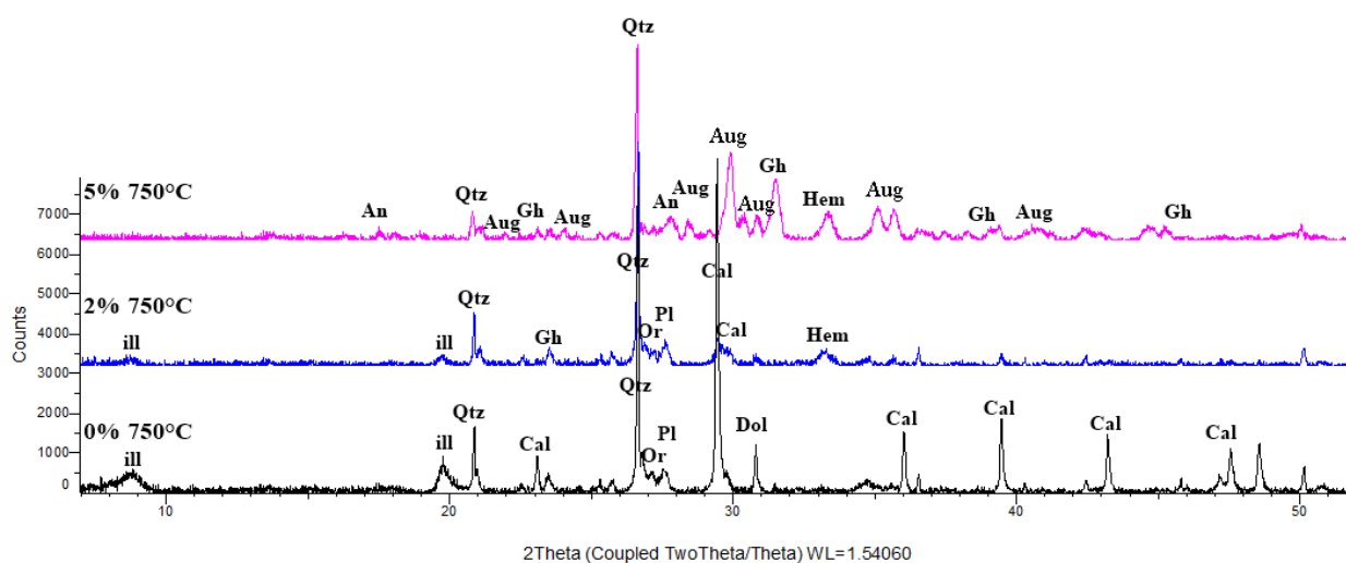
Fig. 44 Evolution of mineralogical phases at 750°C, influenced by the percentage of salt
