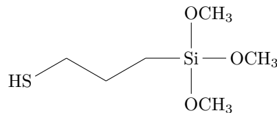
FIGURE 2.4 – 3-Mercaptopropyltriméthoxysilane (MPTMS)
