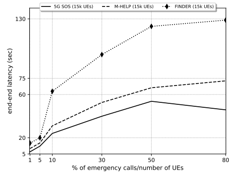
(b) End-end latency against the ratio of NEC to NoU.
