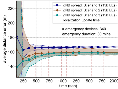
Figure 5.10: Impact of the functioning gNBs distribution over the average distance error (ADE) with MVLA_{all} mode.
