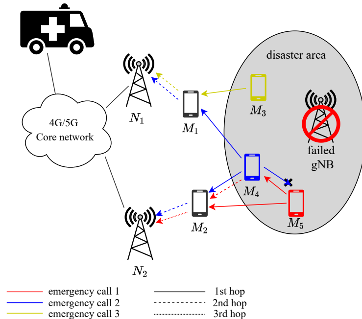
Figure 4.2: The proposed emergency call service architecture. Emergency UEs in the disaster area forward their calls in the direction of the functioning gNBs via relay UEs in the neighborhood. Distinct emergency calls generated by each emergency UE are represented by the color of the arrow. Solid lines indicate the D2D communication mode, while dashed lines indicate the classical communication between gNB and UE.
