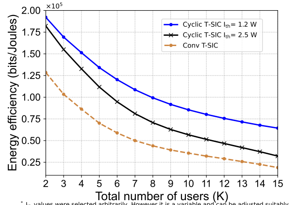
(b) EE vs total number of users under varying I_{th} . Parameters: \nu = 5 , \phi = 50\% .
