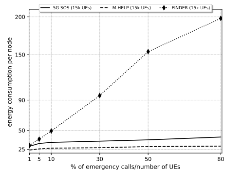
(d) Energy consumption per node against the ratio of NEC to NoU.
