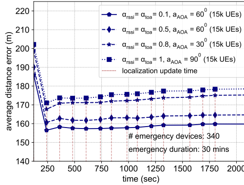
(c) Comparison of ADE against time under different \alpha_{RSSI} , \alpha_{ToA} , \alpha_{AoA} values in MVLA_{all} mode. Localization scheme: GPS+RSSI+AoA+ToA.
