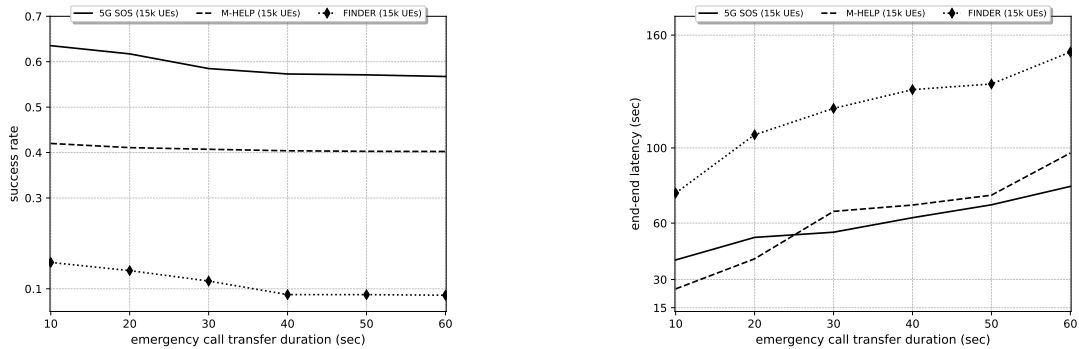
(a) Success rate against emergency call transfer duration.
