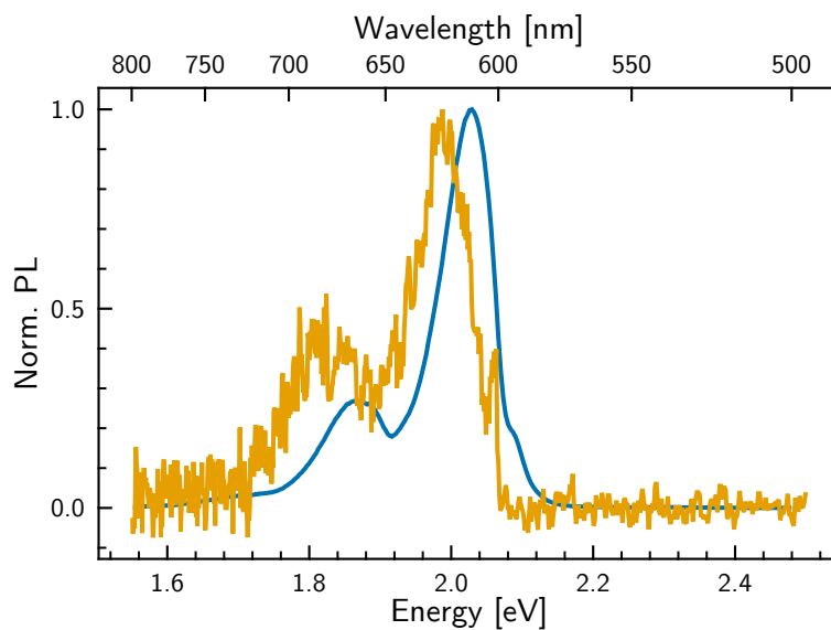
Figure 4.15: Emission spectra of C_{96}tBu_8 in solution (blue) and of a single impurity in the polystyrene matrix (yellow).
