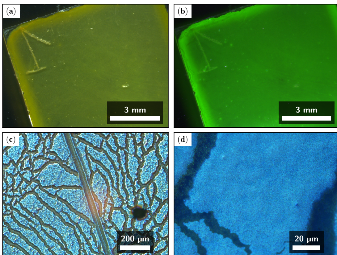
Figure 3.14: (a) Film of drop-casted nanocrystals. (b) Film of drop-casted nanocrystals under UV illumination. (c) Optical microscopy image of a drop-casted nanocrystal film. The oblique straight line has been manually carved for profilometry measurements. (d) Close-up picture of the film, showing the "cracks" surrounding more uniform areas.
