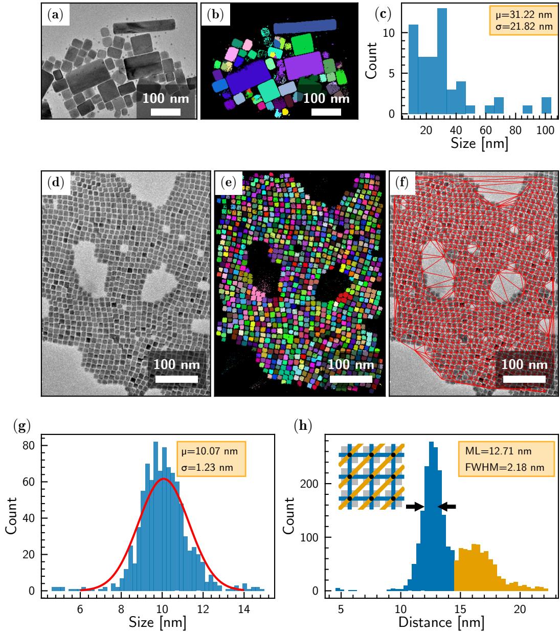
Figure 3.7: (a) TEM image of PVK-TOA. (b) TEM image of PVK-TOA labelled by the watershed algorithm. (c) Histogram of sizes calculated from the TEM image of PVK-TOA. (d) TEM image of nanocrystals. (e) TEM image of nanocrystals labelled by the watershed algorithm. (f) Delaunay triangulation graph of the labelled nanocrystals crystals. (g) Histogram of sizes calculated from the TEM image of nanocrystals. The mislabelled crystals that actually correspond to several nanocrystals visible in (e) have been removed from the dataset. (h) Histogram of distance between nodes in the triangulation graph of nanocrystals, i.e. distance between the centers of the nanocrystals. The inset shows the triangulation on an idealized infinite square grid, and the color code of the edges corresponds to the color code on the histogram. FWHM, Full Width at Half Maximum, ML, Maximum of Likelihood.
