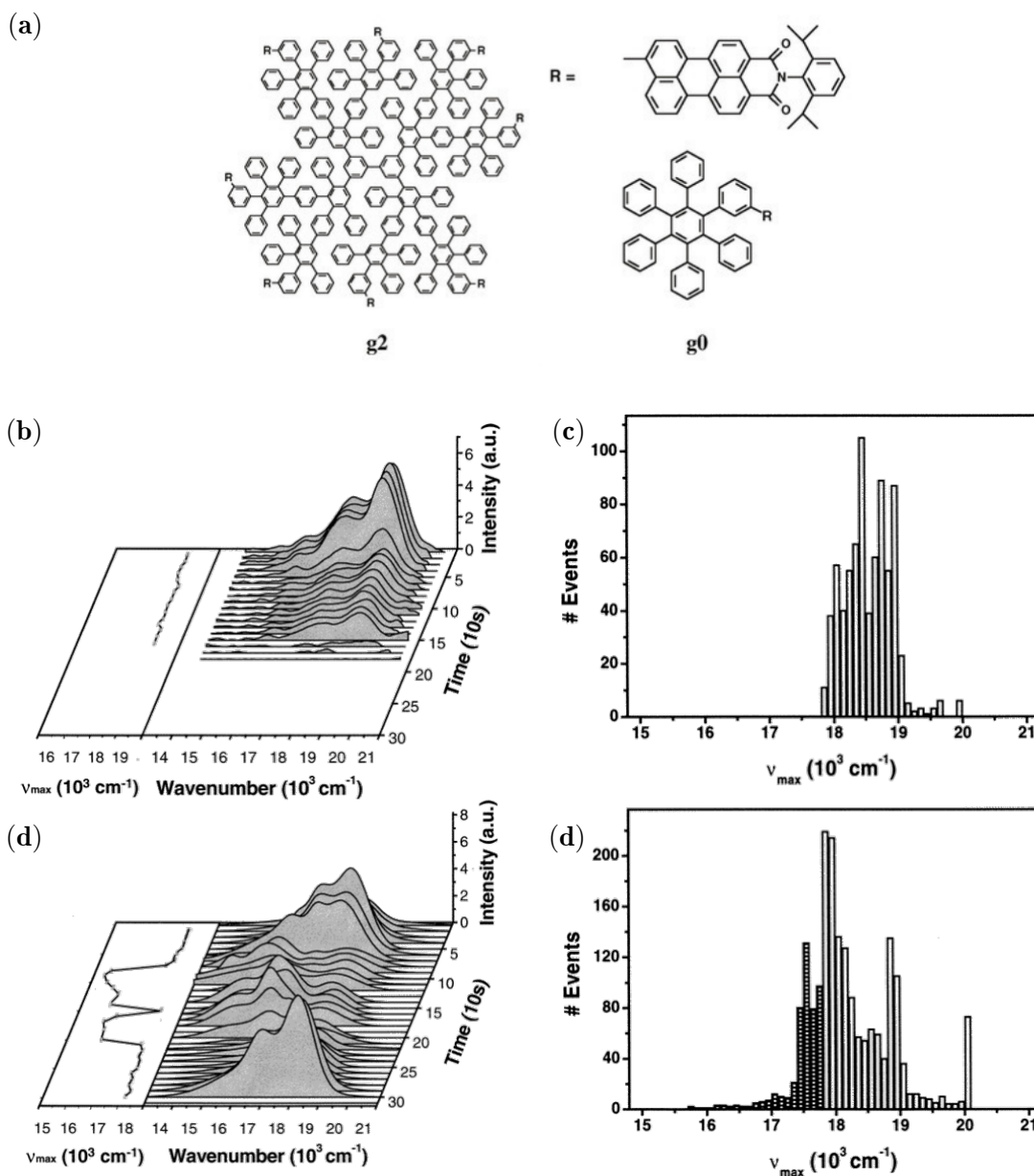
Figure 5.24: (a) Molecules studied by Hofkens et al. [288]. g0 is a small dendrimer functionalized with a unique chromophore, while g2 corresponds to a bigger dendrimer functionalized with eight chromophores. (b) Evolution of the emission spectra of g0 over time. (c) Histogram of the positions of the maximum of photoluminescence for g0 . (d) Evolution of the emission spectrum of g2 over time, featuring discrete jumps towards lower energy regions. (e) Histogram of the positions of the maximum of photoluminescence for g2 . The histogram shows a broader distribution towards lower energies, corresponding to spectra jumps to these regions. Reproduced from Ref. [288].
