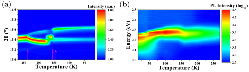
Figure 1.11: (a) Detailed X-Rays diffraction spectra of a MAPbBr 3 single crystal as a function of temperature. Three phase transition points are identified at \sim 230 K, \sim 160 K, and \sim 150 K, corresponding to transitions from cubic to tetragonal and finally orthorhombic phases. (b) Temperature-dependent photoluminescence spectrum of a MAPbBr 3 single crystal. Reproduced from Ref. [40]
