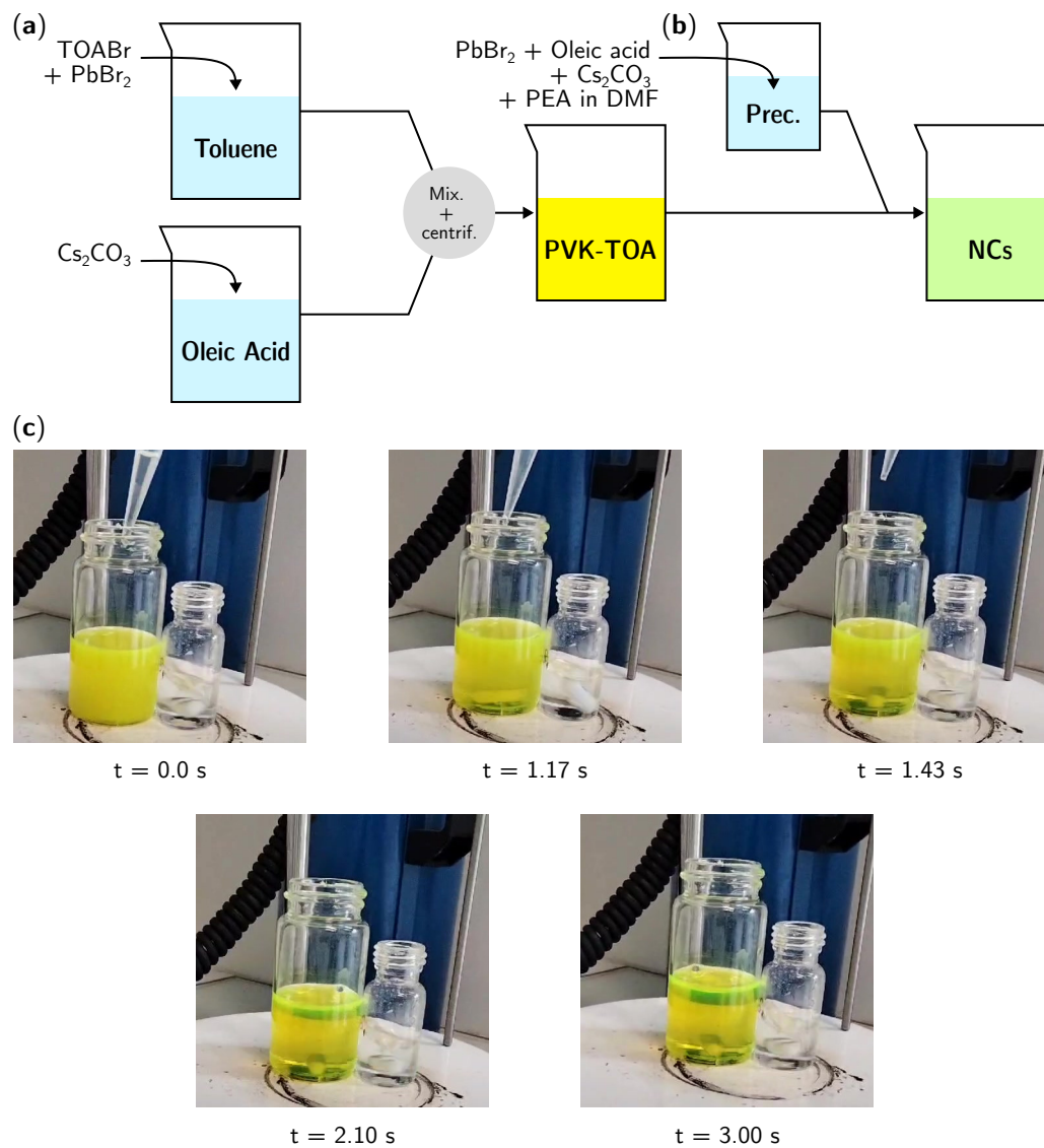
Figure 3.5: Schematic representation of the synthesis of (a) PVK-TOA, and then (b) \text{CsPbBr}_3 nanocrystals. (c) Excerpt of a video showing the PVK-TOA in solution being cut into \text{CsPbBr}_3 nanocrystals. The full video is available at https://media.hal.science/hal-04310797 .
