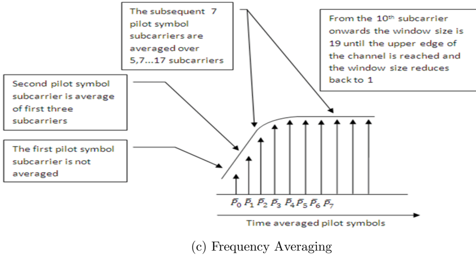
Figure 3.6: Channel Estimation over PRS
