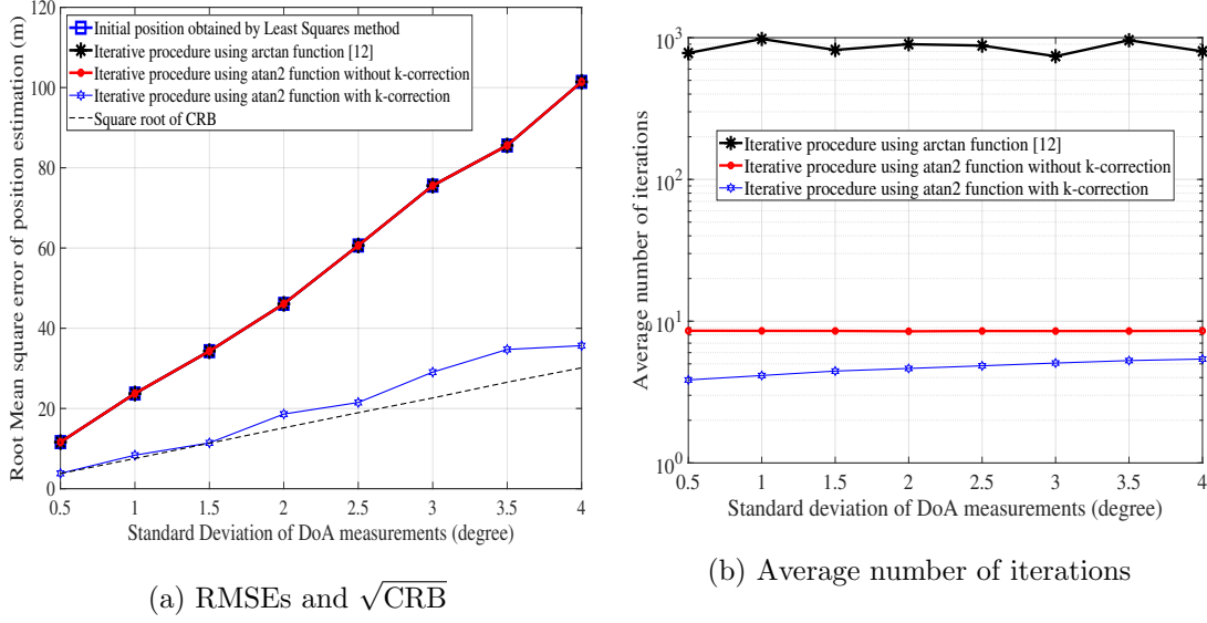
Figure 5.5: Comparisons among the algorithms when N = 8 BSs, standard deviation of DOA measurements varies from 0.5^\circ to 4^\circ
