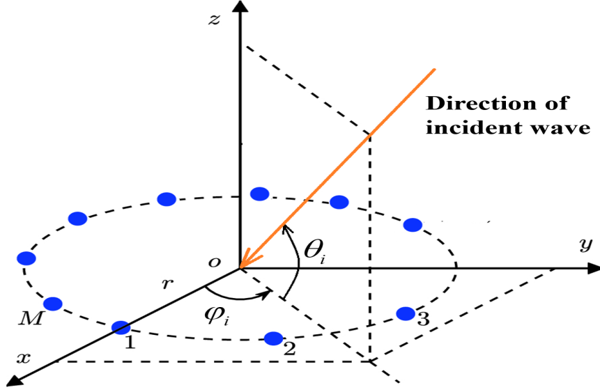
Figure 4.3: M -element Uniform Circular Array (UCA) with radius r at the i -th base station to estimate azimuth angle \varphi_i and elevation angle \theta_i
