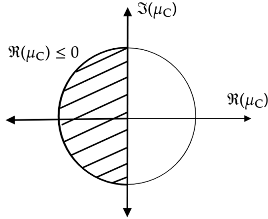
Figure 2.9: The shaded region of consideration where \Re(\mu_{\mathbf{C}}) \leq 0
