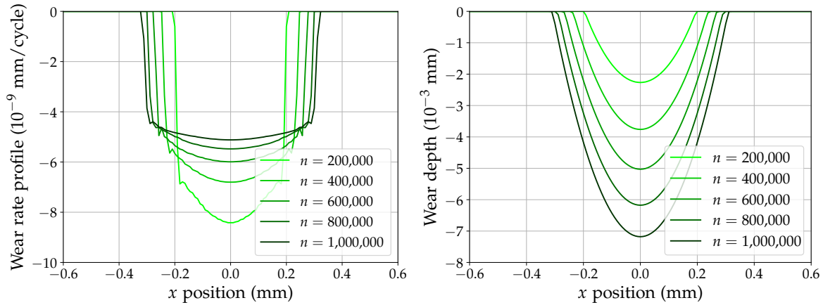
(a) Wear rate profiles
