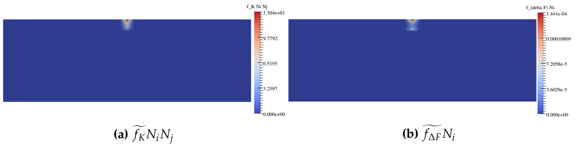
Figure B.7: Fields \widetilde{f}_K N_i N_j and \widetilde{f}_{\Delta F} N_i at time step t_{j+1} .
