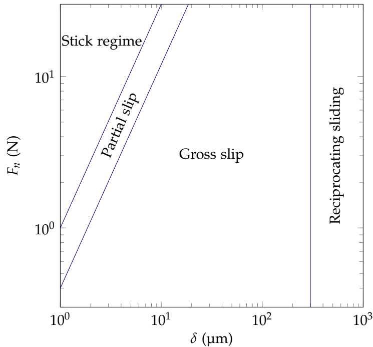
Figure 1.7: Example of fretting map as a function of normal load and displacement amplitude [Vingsbo and Söderberg 1988].
