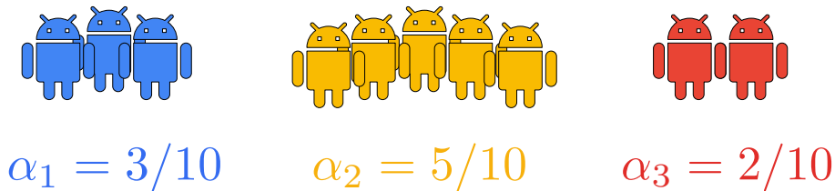
Figure 2.3: Example with three subpopulations and \boldsymbol{\alpha} = (0.3, 0.5, 0.2) \in \Sigma_3 .
