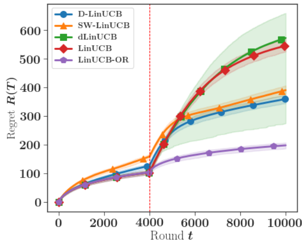
Figure 4.2: Behavior of the different algorithms on large-dimensional data
