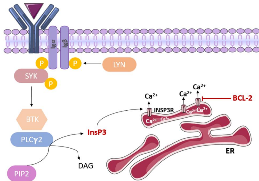
Figure 16: Ca^{2+} mobilization via BCR signaling. PLC \gamma 2 is activated by BTK following BCR stimulation. It cleaves PIP2 into InsP3 and DAG. INSP3 binds to its ER receptor INSP3R, causing the release of calcium. ER Ca^{2+} release can be suppressed by the anti-apoptotic protein BCL-2.
