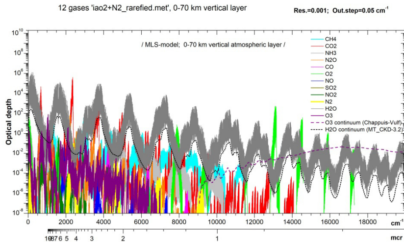
Fig. 3. (Courtesy of I. Ptashnik and A. Simonova) Optical depth for the main atmospheric gases.
