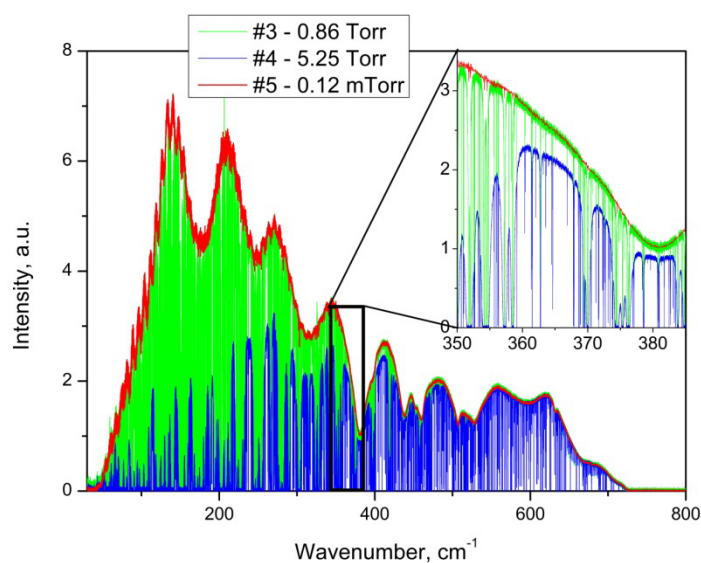
Fig. 2.4. “Raw” FTS spectra #3, #4 and #5.
