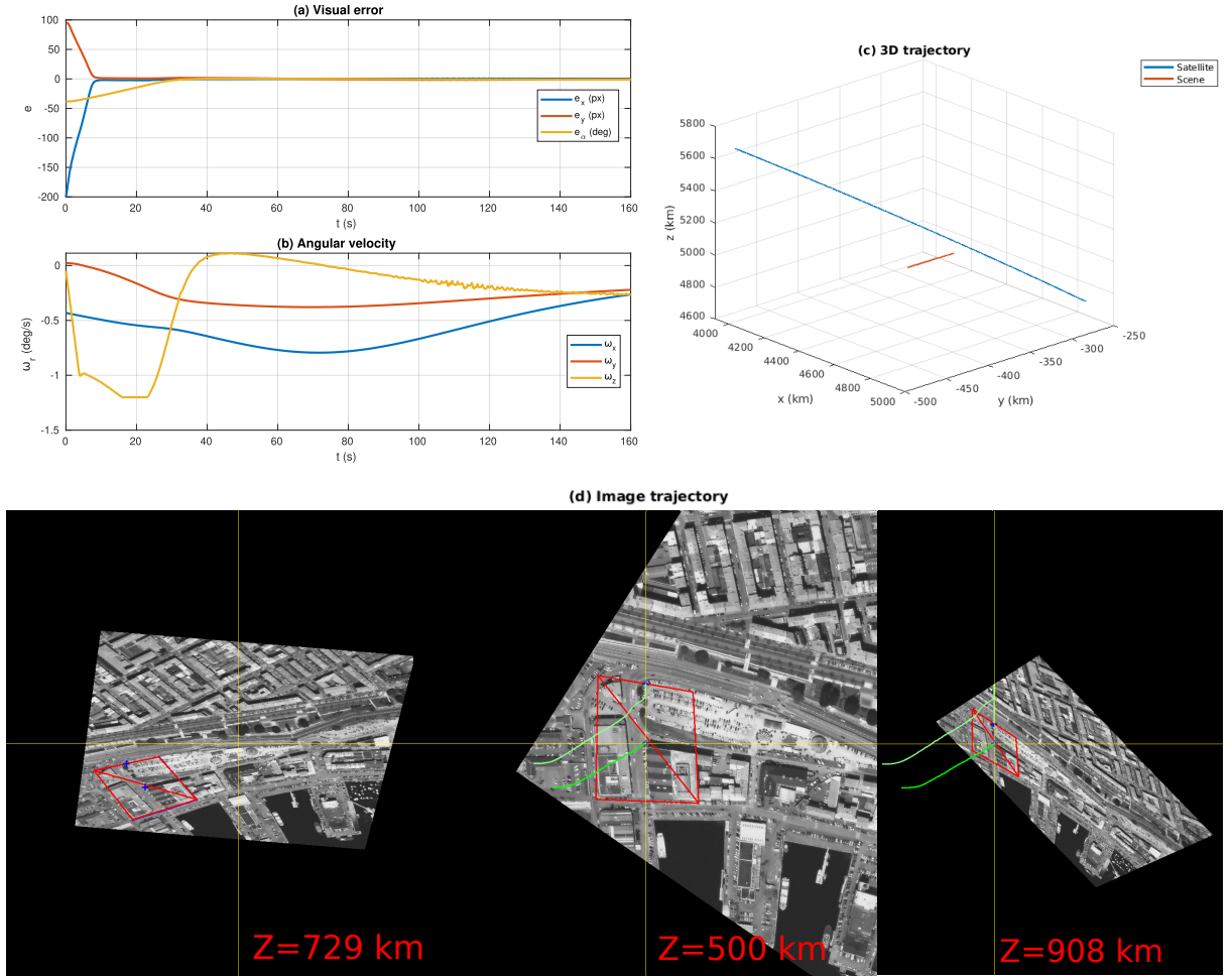
Figure 3.10 – Control law results in the same configuration as Figure 3.9 but the gain \lambda_\alpha is increased, which enhances the convergence time of the orientation task against stronger saturations on the z axis, which have no visible impact on the image trajectory. A video illustrating the results is available here .
