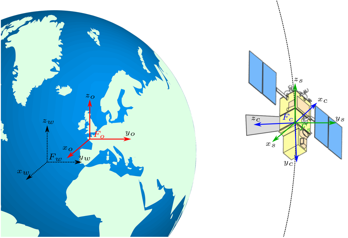
Figure 3.1 – Modeling of the system: a camera embedded on a satellite F_c is directed by the uncontrolled orbital translations induced by its orbit at the center of mass of the satellite F_s , and controlled in rotations to track a terrestrial object of interest F_o . The world frame F_w corresponds to the Earth-Centered Inertial frame of reference.
