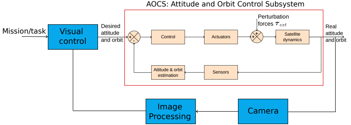
Figure 2.8 – Satellite vision-based control loop
