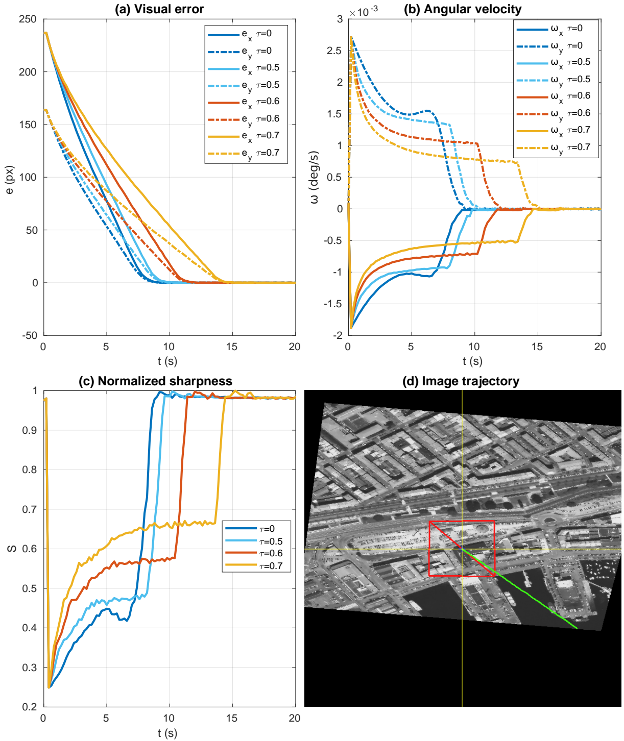
Figure 4.10 – Non-predictive constraint (4.45) applied to the fixed pan-tilt configuration tracking a location in the port of Brest, wrt. \tau . S^* = 393.2 . The image trajectory is all the time a perfect straight line.
