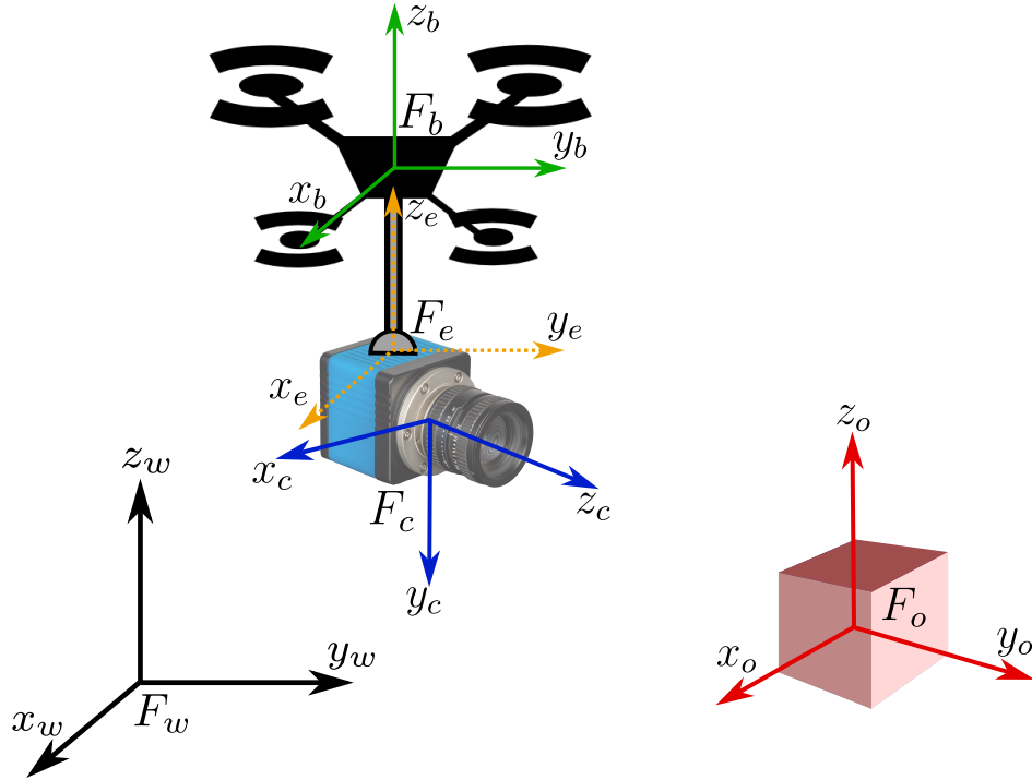
Figure 1.9 – Camera embedded on a moving vehicle (here a drone). Among the common frames F_w , F_c and F_o , the frame F_b is attached to the body of the drone and the frame F_e corresponds to the end effector frame which is here a pan-tilt-roll unit.
