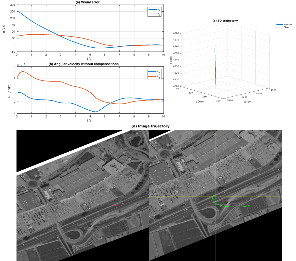
Figure 3.14 – Control law results considering a moving car in a sequence of images of Barcelona. A video illustrating the results is available here . The car is successfully tracked and centered thanks to the adaptive visual integrator that cancels the tracking error, visible from the first inflection point. The angular velocity is shown without the compensation of orbital and terrestrial motions, so the influence of the feedback term and of the integrator are highlighted.
