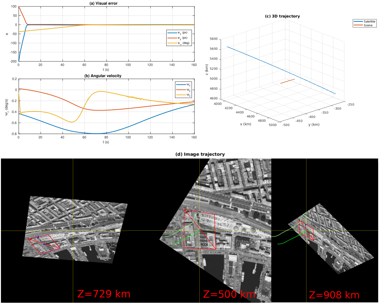
Figure 3.9 – Control law results considering the same object of interest as Figure 3.8 and with exactly the same gains. A video illustrating the results is available here . The results are similar in terms of convergence time and angular velocity, but the image trajectory is not a perfect straight line at the beginning.
