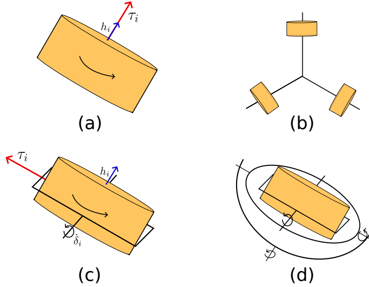
Figure 2.6 – Principles of reaction wheel and control moment gyroscope, (a) RW exerting a torque \tau_i = \dot{h}_i with h_i the angular momentum of the rotating wheel, (b) Composition of RWs to control 3 rotational axes, (c) CMG exerting a torque \tau_i = \dot{\delta}_i \times h_i with \dot{\delta}_i the angular speed of the gimbal, (d) CMGs: a 3 DOF gimbal to orientate the rotating wheel and so the resulting torque.
