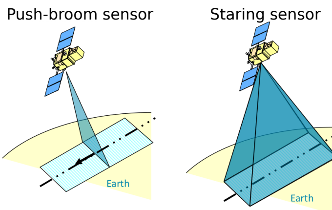
Figure 2.13 – Push-broom and staring sensors.
