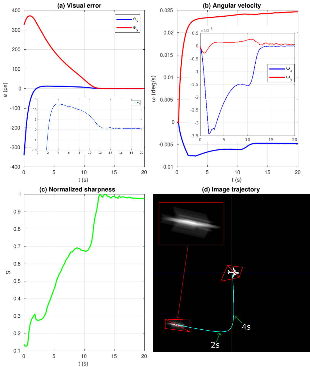
Figure 4.13 – Predictive constraint (4.54) applied to the pan-tilt satellite configuration tracking an airplane flying at 800 km/h above water. S^* = 523.2 . Velocity in (b) are subtracted from orbital motion compensations, the inner figure also subtracts the compensation for the airplane motion.
