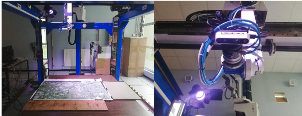
Figure 3.15 – AFMA Cartesian robot positioned above a satellite image, and its INTEL D435 camera mounted on a pan-tilt-roll unit.
