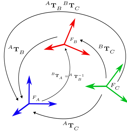
Figure 1.1 – Frame transformations
