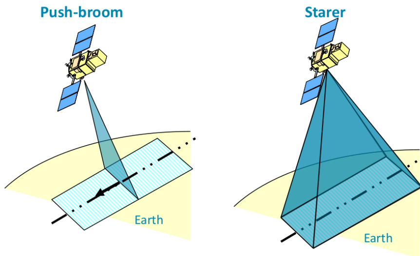
Figure 1 – Push-broom and starrer technologies
