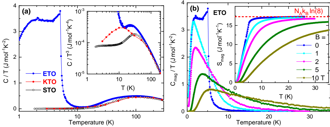
Fig. 5.11 Specific heat in three quantum paraelectric solids: a) Temperature dependence of the total specific heat in K\text{TaO}_3 , \text{SrTiO}_3 and \text{EuTiO}_3 plotted as C/T vs. T . The inset is an enlarged view of the same data shown as \frac{C_p}{T^3} vs. T . Note the presence of Einstein modes in all three solids and the additional magnetic specific heat in ETO emerging below 15 K. b) Evolution of C_{\text{mag}}/T of ETO for different magnetic fields up to 10 T. The inset shows the corresponding magnetic entropy S_{\text{mag}} = \int C_{\text{mag}}/T dT of ETO and the maximum magnetic entropy N_A k_B \ln(2S + 1) of a spin 7/2 system is indicated by the dashed line.
