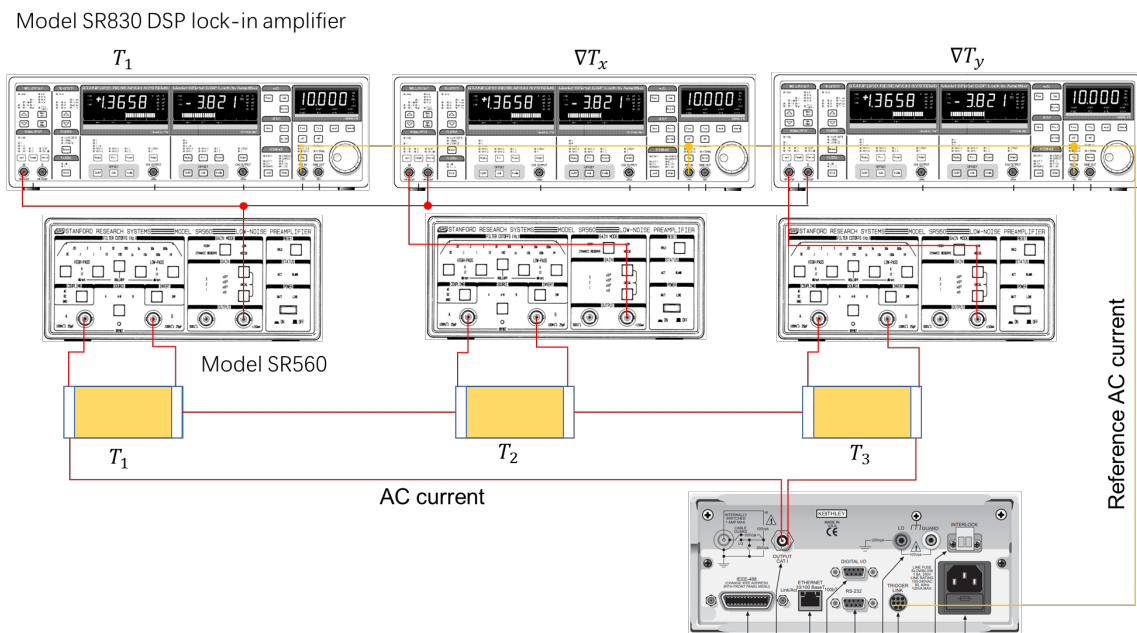
Fig. 1.5 Measurement of temperature and temperature difference using three thermometers (Cernox 1030 or RuO 3 chip resistor). The AC current provided by Model 6221 passes through the three thermometers. The AC voltage of each three thermometers is first amplified by the Model SR560 preamplifier and then detected by the Model SR830 lock-in amplifier. The voltage difference between T 1 and T 2 (T 1 and T 3 ) is measured to have a high-precision temperature difference signal ∇T x (∇T y )
