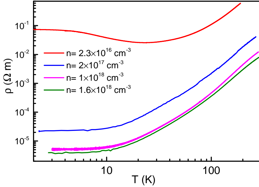
Fig. 3.5 Electrical resistivity ( \rho ) as function of temperature for \text{SrTiO}_{3-\delta} samples with different carrier concentrations.
