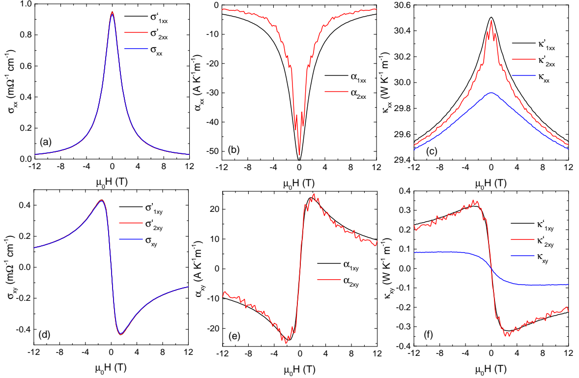
Fig. 3.14 (a)-(c) Longitudinal electric ( \sigma_{xx} ), thermoelectric ( \alpha_{xx} ) and thermal conductivity ( \kappa_{xx} ) as a function of field at T = 19.4 K for \text{SrTiO}_{3-\delta} ( n = 1 \times 10^{18} \text{ cm}^{-3} ). The black and red colors correspond to two different combinations of Eq. 3.5, 3.6, 3.7, and 3.8. Black (red) line results were obtained using Eq. 3.5(3.6) 3.6(3.7) and 3.7(3.8). (d)-(f) same as (a)-(c) but for the transverse components of \bar{\sigma}' , \bar{\alpha} and \bar{\kappa}' .
