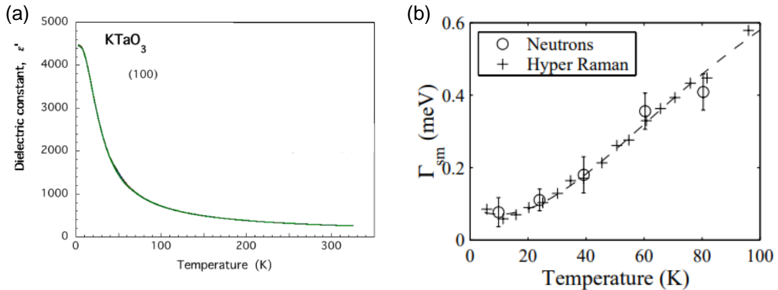
Fig. 2.9 (a) Dielectric constant \epsilon' of \text{KTaO}_3 along [100] as a function of heating temperature [100]. (b) the energy damping of soft zone center TO -mode by neutrons and hyper-Raman measurements [99].
