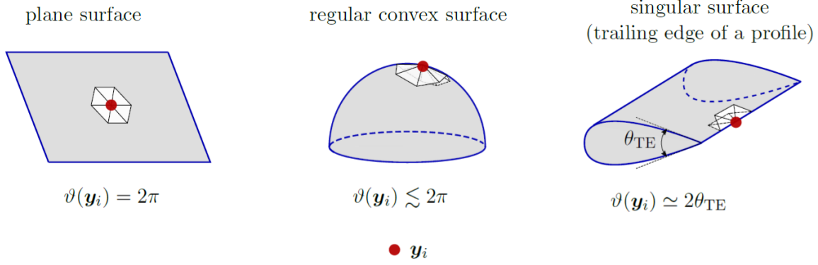
Figure III.1: Value of the solid angle \vartheta associated with the mesh of surfaces with various geometry regularity. The mesh of a plane surface is smooth, the mesh of a regular convex surface (here a sphere) is slightly singular at the node, while the mesh of a profile is strongly singular at the trailing edge. The symbol \lesssim stands for "slightly less than". For a regular concave surface, one would get \vartheta(\mathbf{y}_i) \gtrsim 2\pi .
