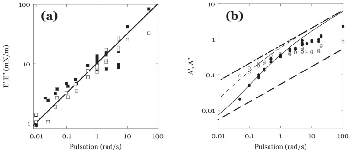
Figure 24: (a) Dilatational moduli of a single interface as function the pulsation. Closed squares for the elastic modulus E' , open squares for the viscous modulus E'' . The line is a model by Lucassen [80]. (b) Elastic and loss moduli of the elementary liquid foam. Closed circles for A' , open circles for A'' . Credits to Besson et al. [78]
