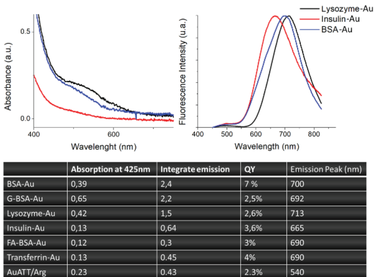
Figure 4.12: Linear optical properties of synthesized protein gold NCs, (Top) UV-vis spectra and emission fluorescence (after excitation at 425nm) and (below) table showing parameters to calculate QY using DCM as external reference.
