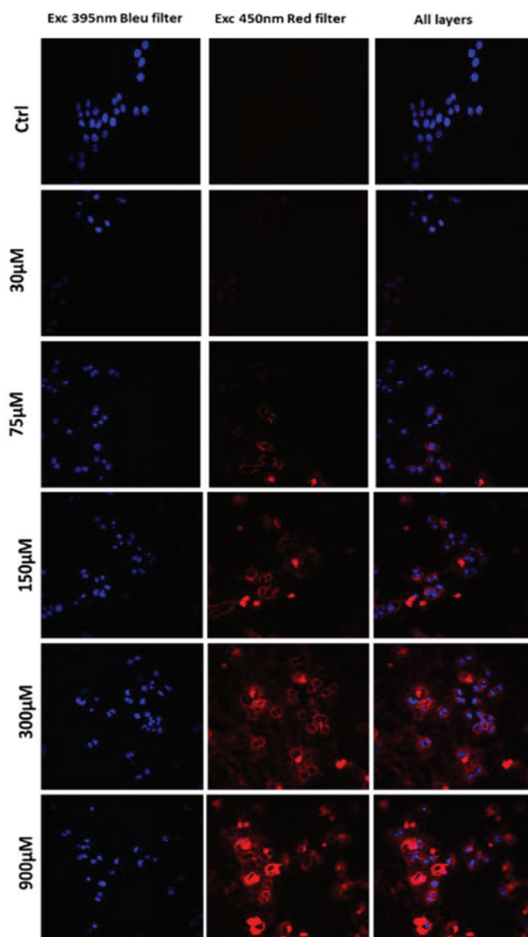
Figure 4.23 : HeLa cells visualized under Nikon spinning disk confocal microscopy incubated with Ag 28 PT 1 DH1A 12 silver NCs for 24h, we dyed the nucleus with DAPI. Removing FBS is better for the internalization of silver NCs for lower concentration up to 30 µM.
