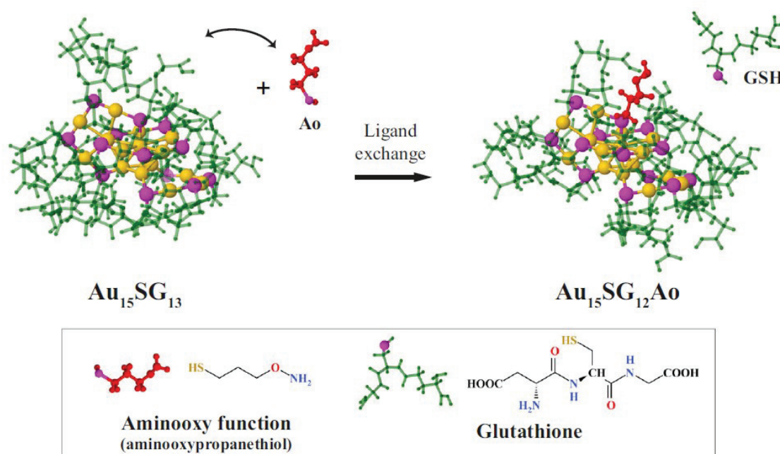
Figure 3.14 : DFT structures illustrate the ligand-exchange strategy to functionalize the NCs with an aminooxy (Ao) function ( \text{Au}_{15}\text{SG}_{12}\text{-Ao} ). We labeled sulfur atoms with magenta, Au-gold, glutathione-green, and aminooxypropanethiol with red.
