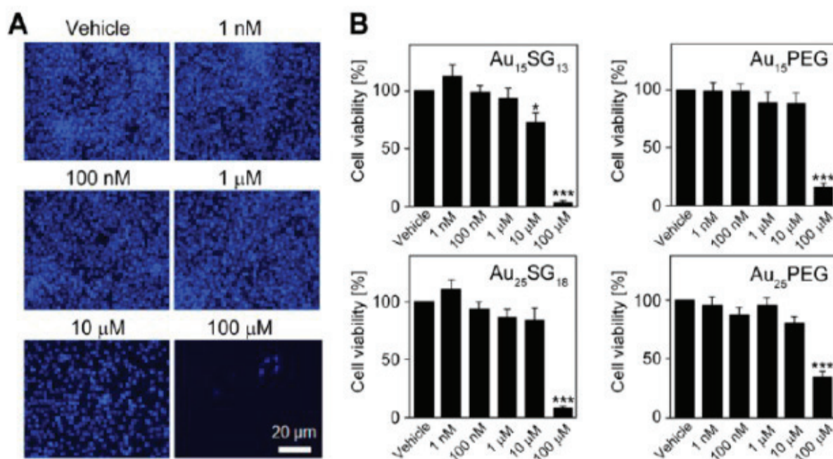
Figure 4.4: (A) U251N human cell treated with different concentration of Au 15 SG 13 for 72 hours, nucleus is stained with Hoechst 33342 to identify cells and (B) Cell number counting compared to vehicle after incubation with the different gold NCs, significant change after treatment with NCs are marked. Maysinger, et al, Gold nanoclusters elicit homeostatic perturbations in glioblastoma cells and adaptive changes of lysosomes. Theranostics , 10(4), 1633-1648. https://doi.org/10.7150/thno.37674 .
