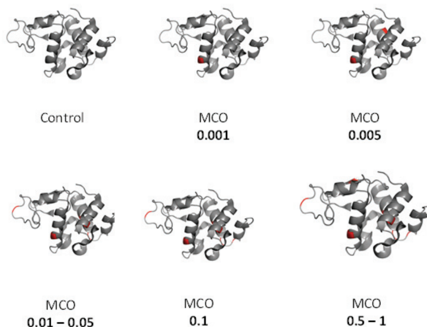
Figure 3.24 : 3D structures of oxidized protein at different doses of MCO oxidation, the carbonylation sites are mostly positioned on the surface of the protein and accessible to functionalized NCs.
