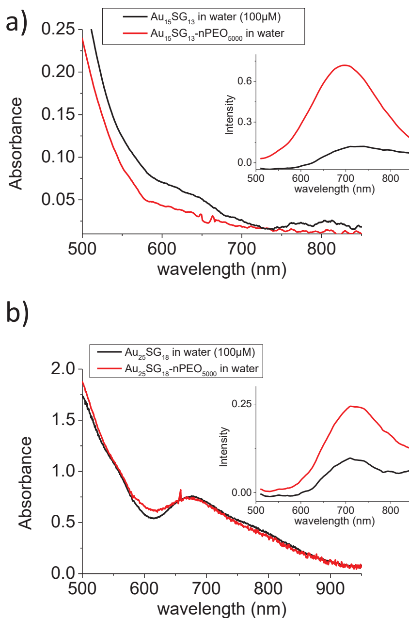
Figure 4.2 : Absorbance and (insets) emission spectra (excitation at 500 nm) of AuSG NCs and PEGylated AuSG NCs in water. a) \text{Au}_{15} and b) \text{Au}_{25} . Maysinger, D., Gran, E.R., Bertorelle, F., Fakhouri, H., Antoine, R., Kaul, E.S., Samhadaneh, D.M., Stochaj, U. (2020). Gold nanoclusters elicit homeostatic perturbations in glioblastoma cells and adaptive changes of lysosomes. Theranostics , 10(4), 1633-1648. https://doi.org/10.7150/thno.37674 .
