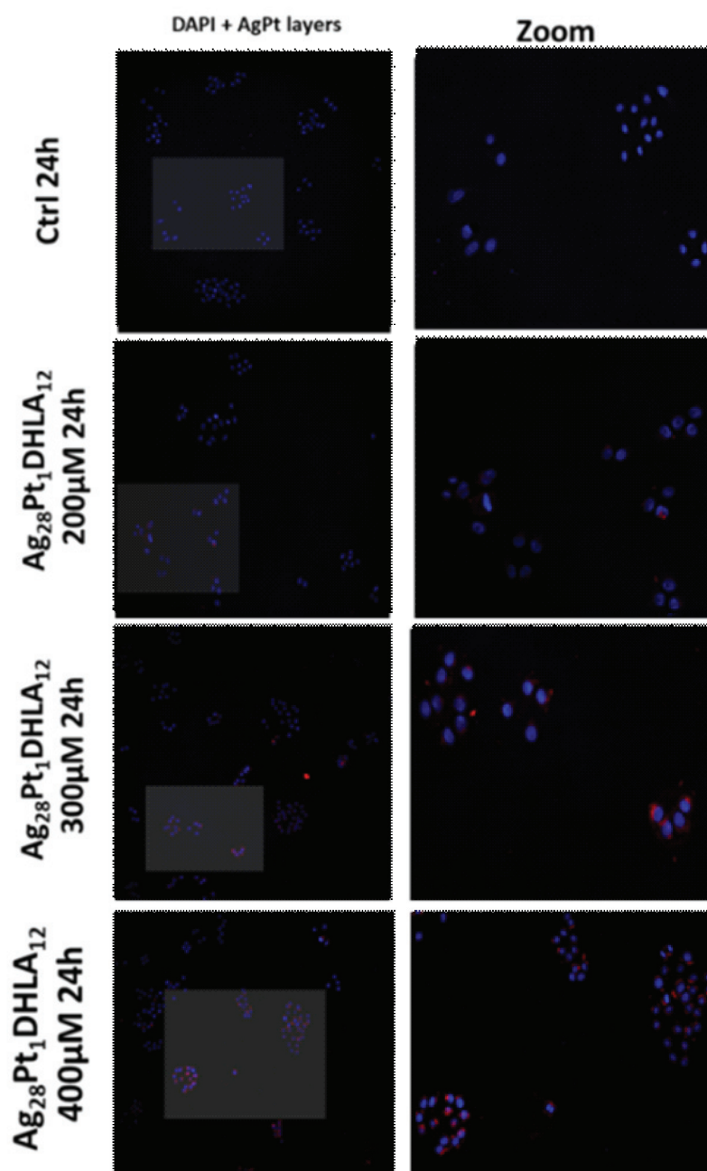
Figure 4.22 : HeLa cells visualized under Nikon spinning disk confocal microscopy incubated with Ag 28 Pt 1 DHCLA 12 silver NCs for 24h, we stained the nucleus with DAPI. In this experiment we dissolved silver NCs in DMEM with FBS which shows after that adding FBS to the medium will limit internalization.
