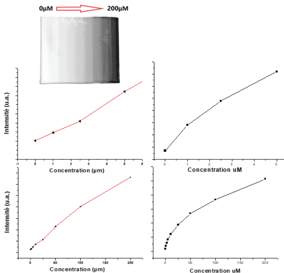
Figure 3.12 : Sensitivity test on dried gel of \text{Au}_{25}\text{SG}_{18} NC collected by multiphoton confocal microscopy (in Red) and by Typhoon TM FLA 9500 biomolecular imager gel scanning system (in black), above shows the data at low concentration to show that both system are sensitive to low concentration of NCs.
