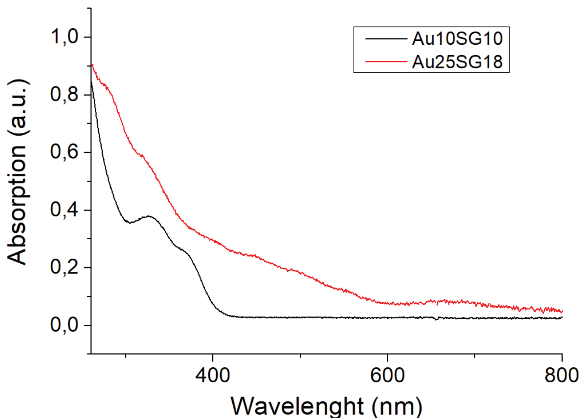
Figure 2.14: Absorption spectra of the \text{Au}_{10}\text{SG}_{10} vs \text{Au}_{25}\text{SG}_{18} , we can see the differences in absorption spectrum between this two NCs.
