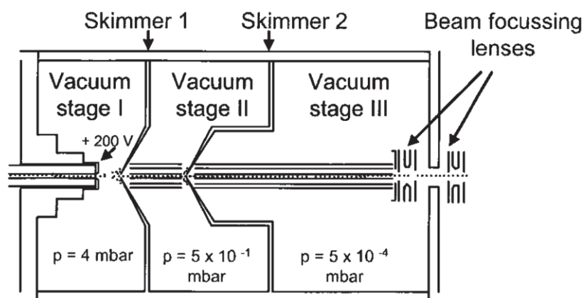
Figure 2.3 : Transfer optics system from microOTOF Bruker
