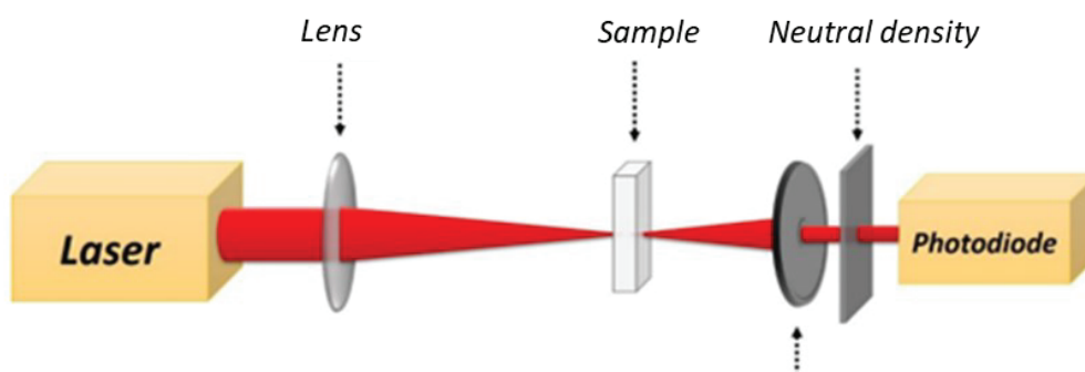
Figure 2.22 : P-scan experimental set-up used to calculate Two Photon Absorption.
