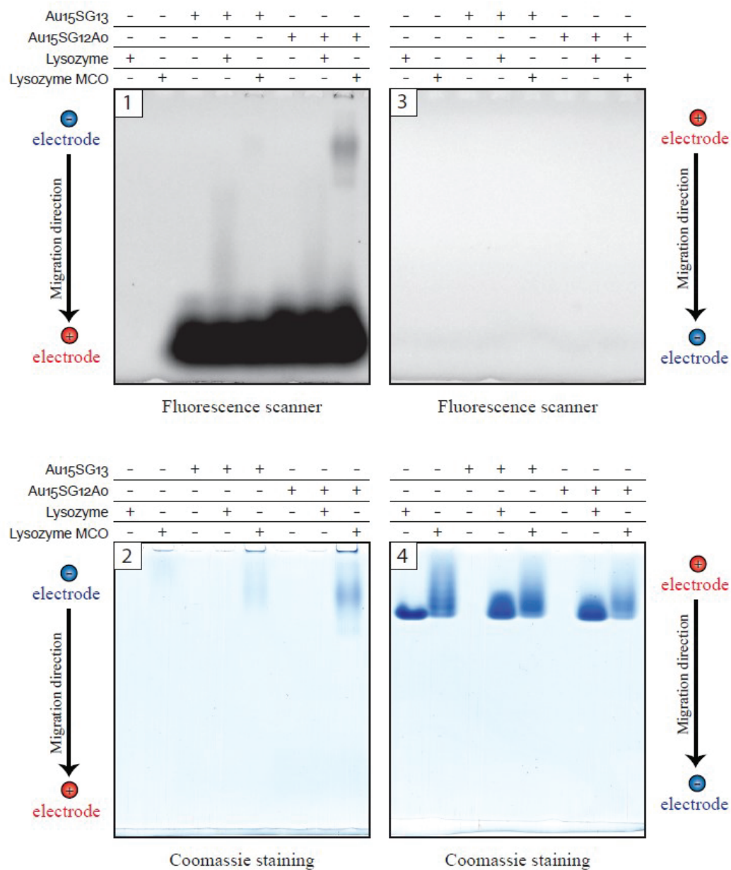
Figure 3.39 : Four identical sets of samples were simultaneously migrated on native polyacrylamide gels with electricity direction from anode to cathode (gels 1 and 2) or from cathode to anode (gels 3 and 4). We dried gels 1 and 3 and stain gels 2 and 4 with Coomassie and scan them under gel scanner.
