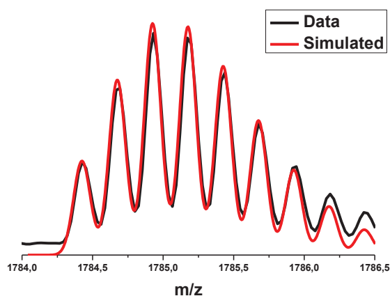
Figure 2.6 : Isotope pattern (black) and isotope pattern simulation (red) for [\text{Au}_{15}\text{SG}_{13}]^{4-} where we used the chemical formula of the molecule, and it is clear that it fits with the experimental results.
