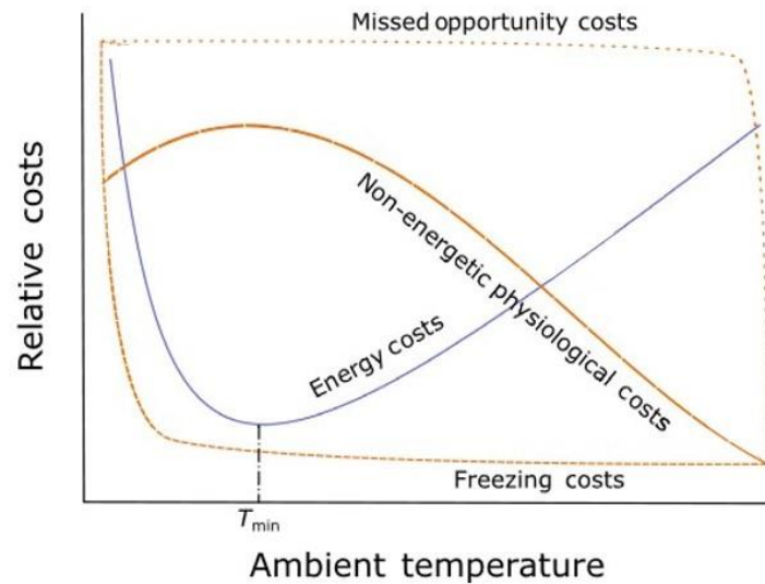
Figure 3. Different relative costs and benefits during hibernation as a function of ambient temperature (proxy of hibernation expression). Whereas energy costs are minimal at minimum ambient temperature, non-energetic physiological costs are maximal at low temperature, and decrease with increasing temperature. Freezing and energy costs increase drastically at low temperature, and the costs of missing opportunities are constant during hibernation (adapted from Boyles et al. 2020).
