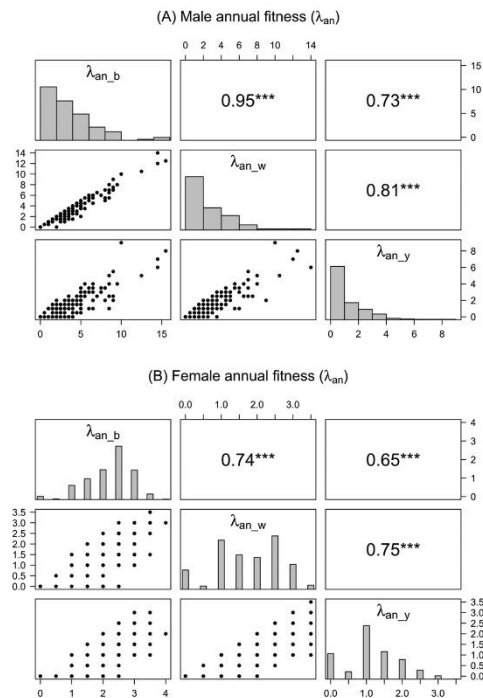
Fig. 1 Pairwise correlation plots for (A) male and (B) female annual fitness metrics calculated from offspring counted at birth ( \lambda_{anb} ), weaning ( \lambda_{anw} ), or surviving to yearling age ( \lambda_{any} ). The distribution of data is given on the diagonal. Significant Spearman's correlation coefficients are given for *** P < 0.001
