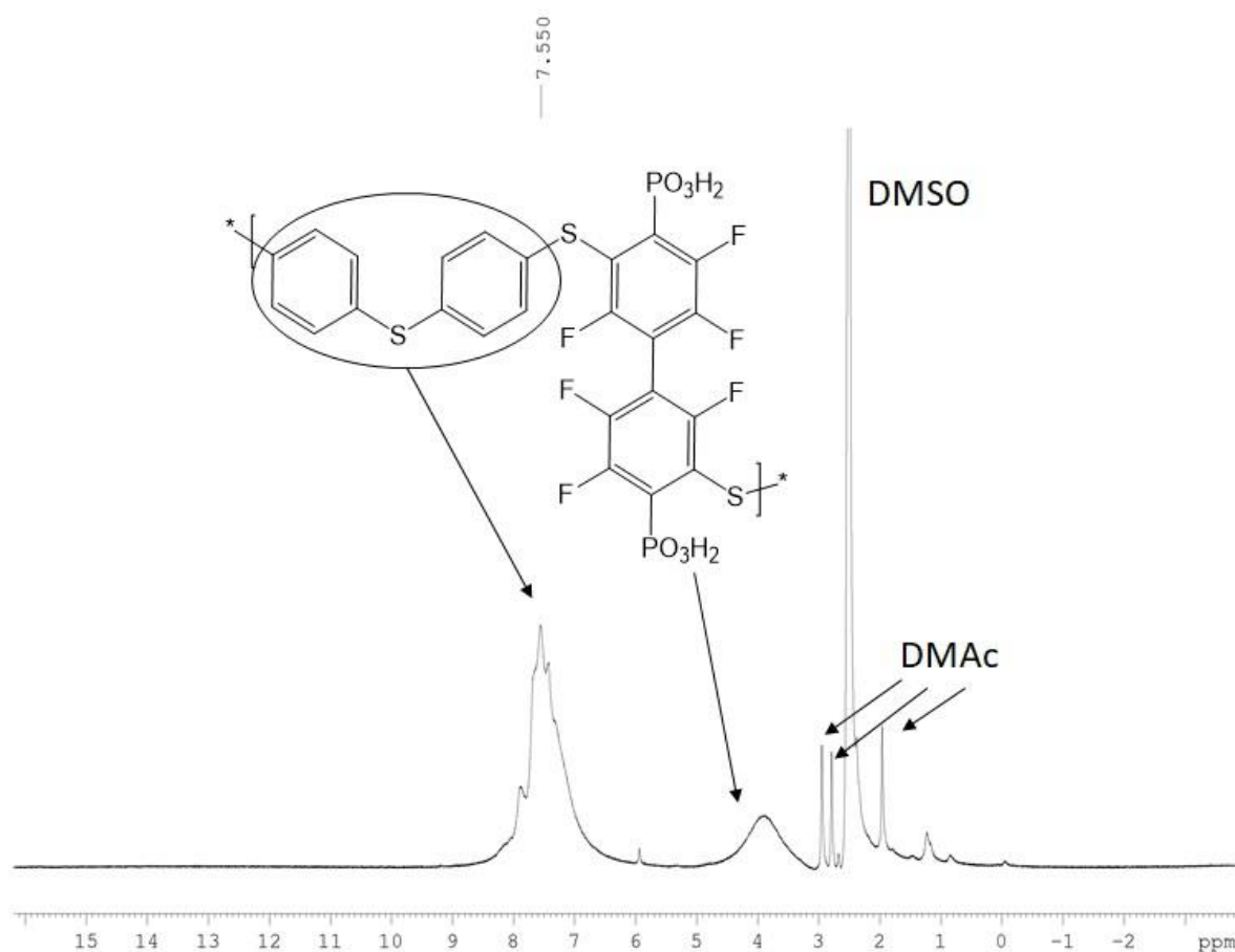
Figure II-37. ^1\text{H} NMR biphosphonated hexafluorinated poly(phenylsulfide)s
