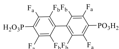
Figure II-14. Phosphonated octafluorobiphenyl
