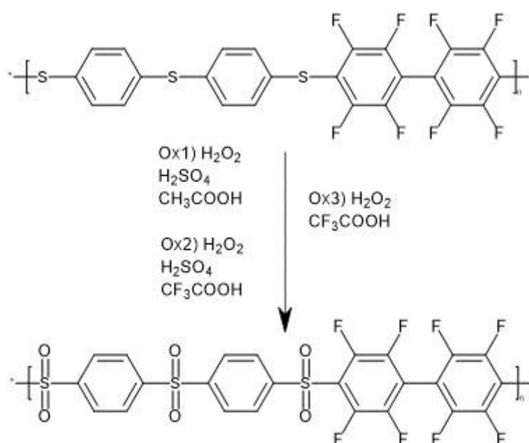
Figure III-22. Oxidation of poly(phenylenesulfide)s scheme.
