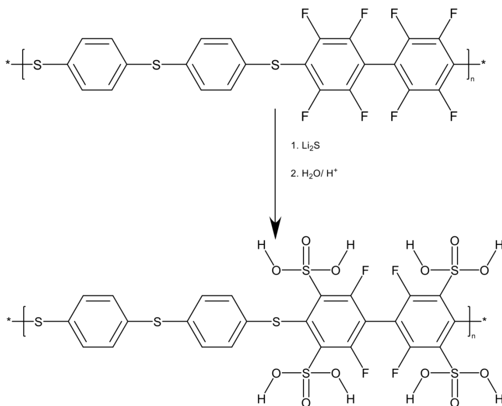
Figure III-12. Sulfonation of fluorinated poly(phenylenesulfide)s using Li 2 S.
