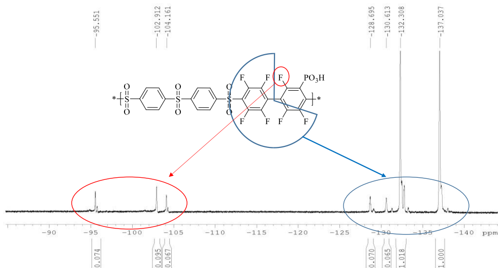
Figure III-28. ^{19}\text{F} NMR phosphonated poly(phenylenesulfone)s.
