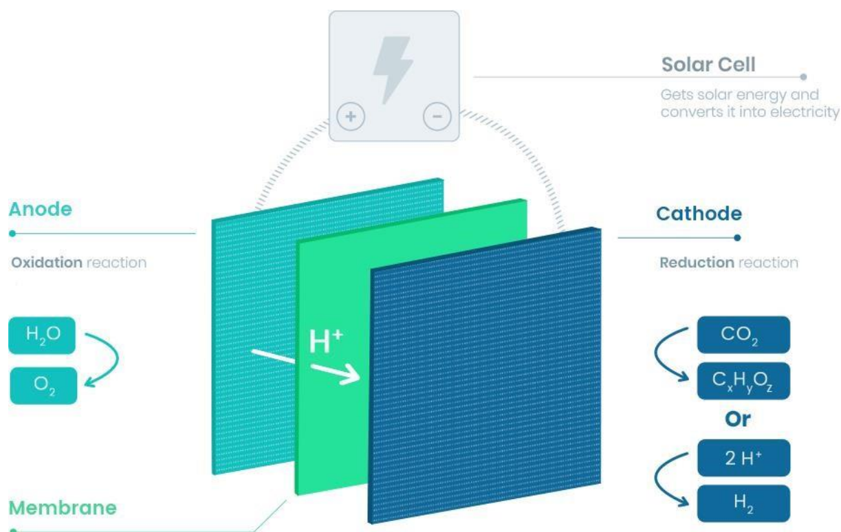
Figure I-2. eSCALED project device scheme.
