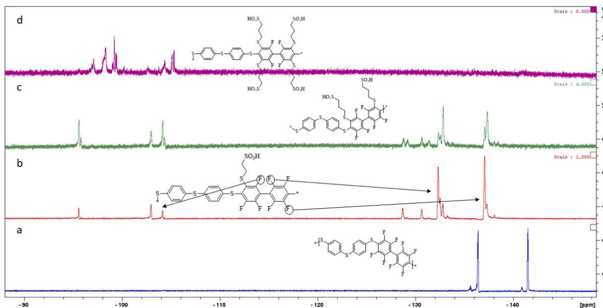
Figure III-41. ^{19}\text{F} NMR polymer with increasing levels of sulphonation.
