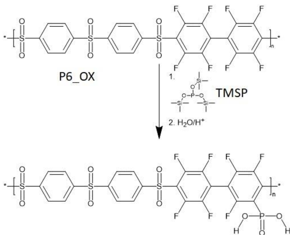
Figure III-9. Phosphonation of fluorinated poly(phenylenesulfone)s.
