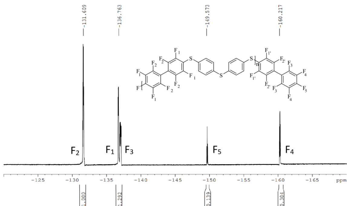
Figure II-26. ^{19}\text{F} NMR of polymerization of DCFB and TMSTB
