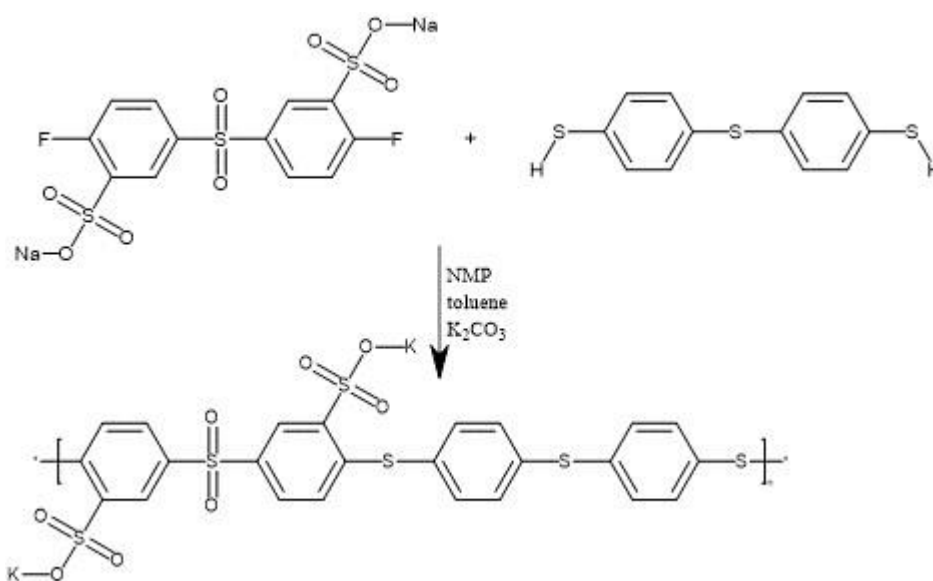
Figure II-38. Polymerization of disodium 3,3'-disulfonate-4,4'-difluorodiphenylsulfone and TBBT
