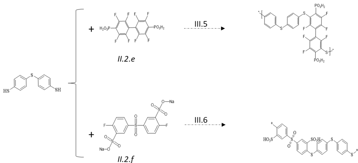
Figure V-3. Scheme of polymerizations starting with 4,4'-thiobisbenzenthrol and prefunctionalized monomers.
