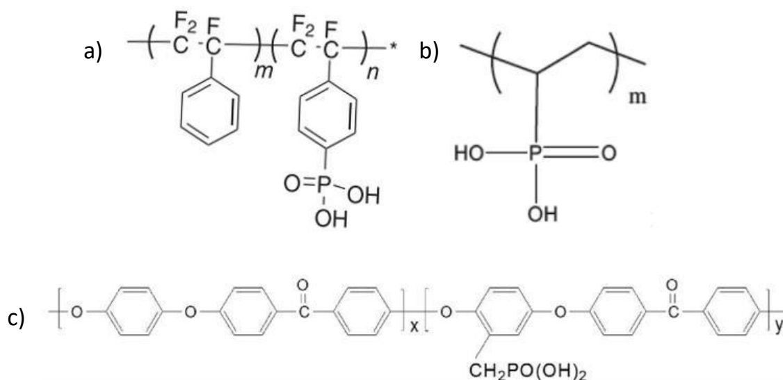
Figure III-1. Dimethyl phosphonate-4-substituted \alpha,\beta,\beta -trifluorostyrene (up-left), PVPA (up-right) and PEEK (down).
