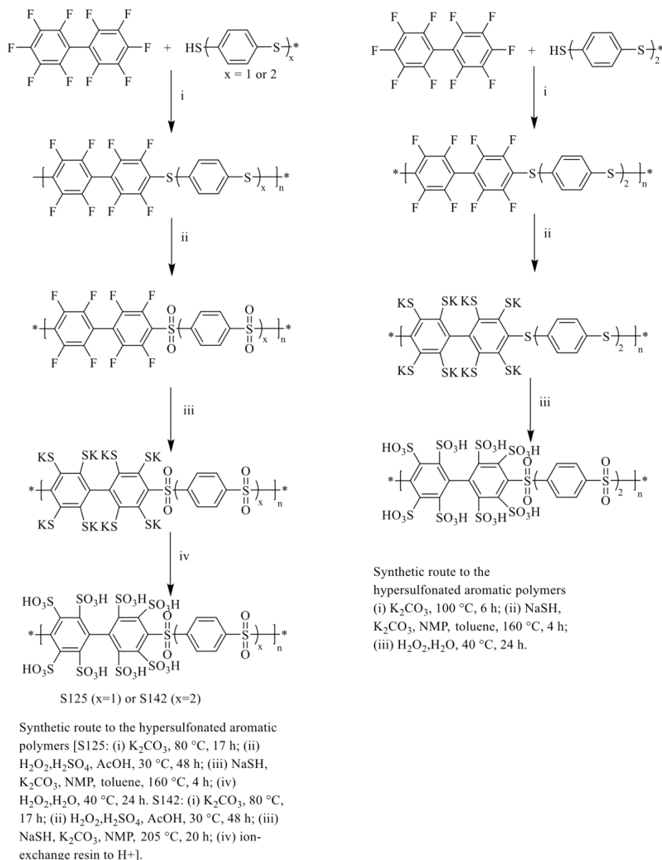
Figure III-30. Polymerization and Sulfonation done by S. Takamuku et al. (left), polymerization and sulfonation done in this thesis.
