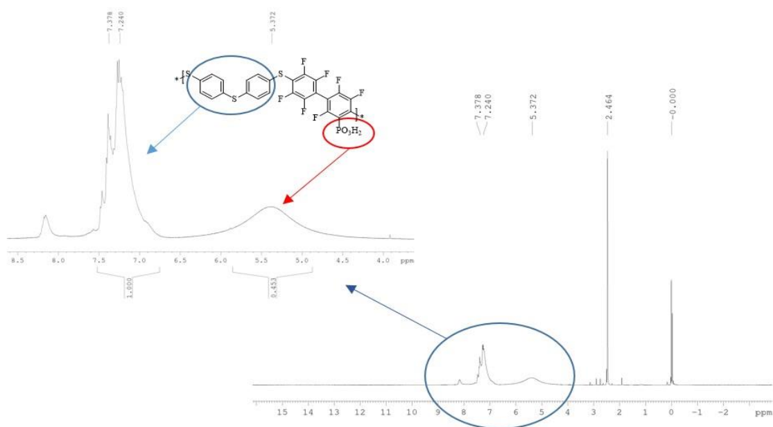
Figure III-19. 1 H NMR phosphonated poly(phenylenesulfide)s.
