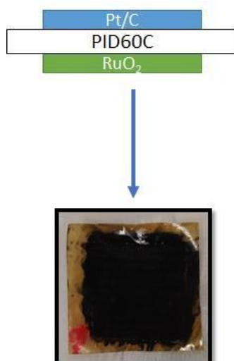
Figure IV-14. Membrane 3x3cm. P4SM-c_CCM after catalyst deposition.
