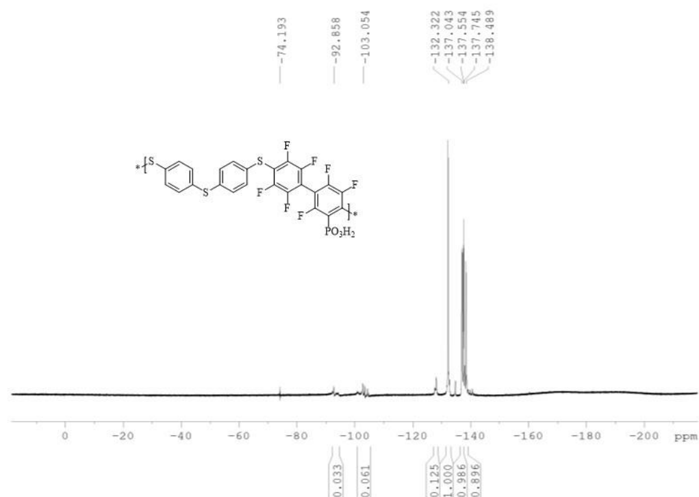
Figure III-18. 19 F NMR phosphonated poly(phenylenesulfide)s
