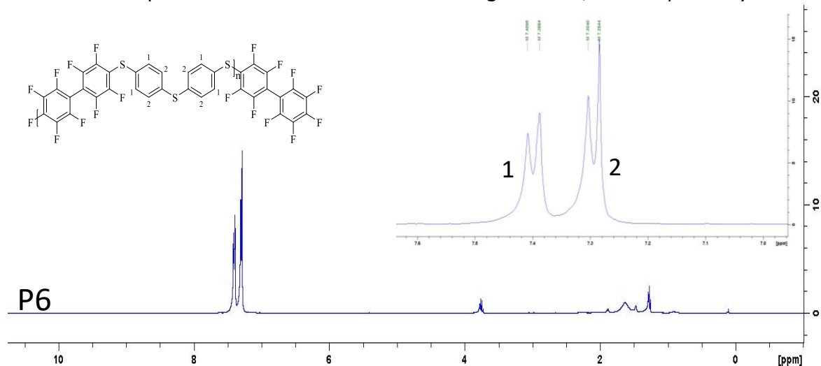
Figure II-21. 1 H NMR P6
