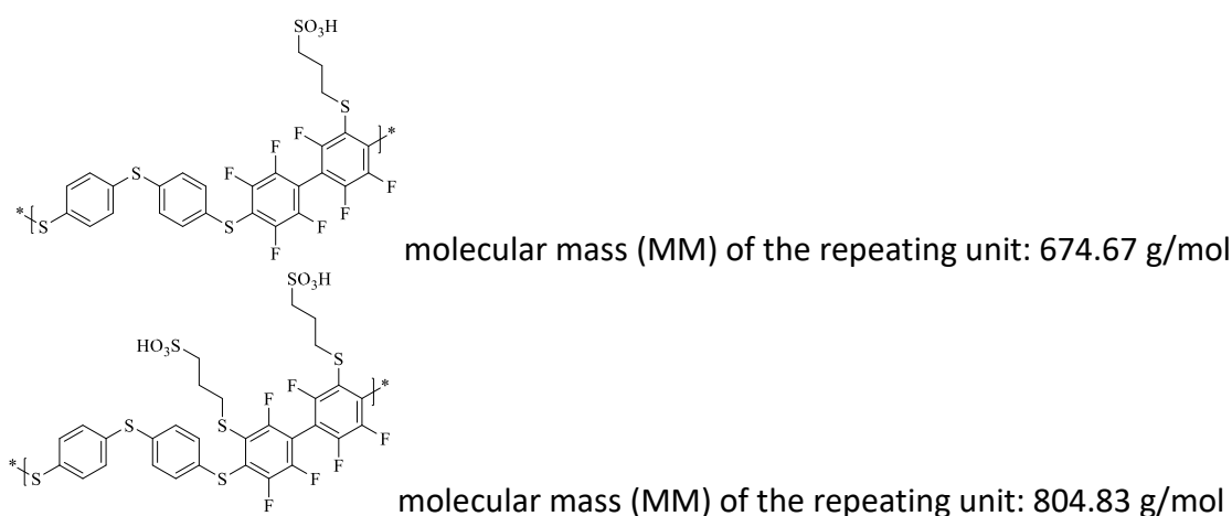
Figure IV-4. P1S and P2S, fluorinated sulfonated poly(phenylenesulfide).
