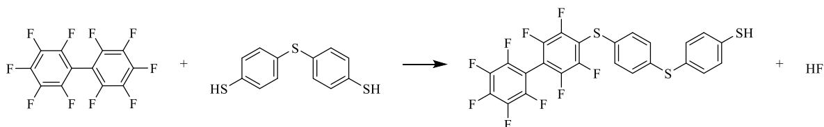
Figure II-7. Polymerization of Decafluorobiphenyl (DFBP) and 4,4'-Thiobisbenzenethiol (TBBT).
