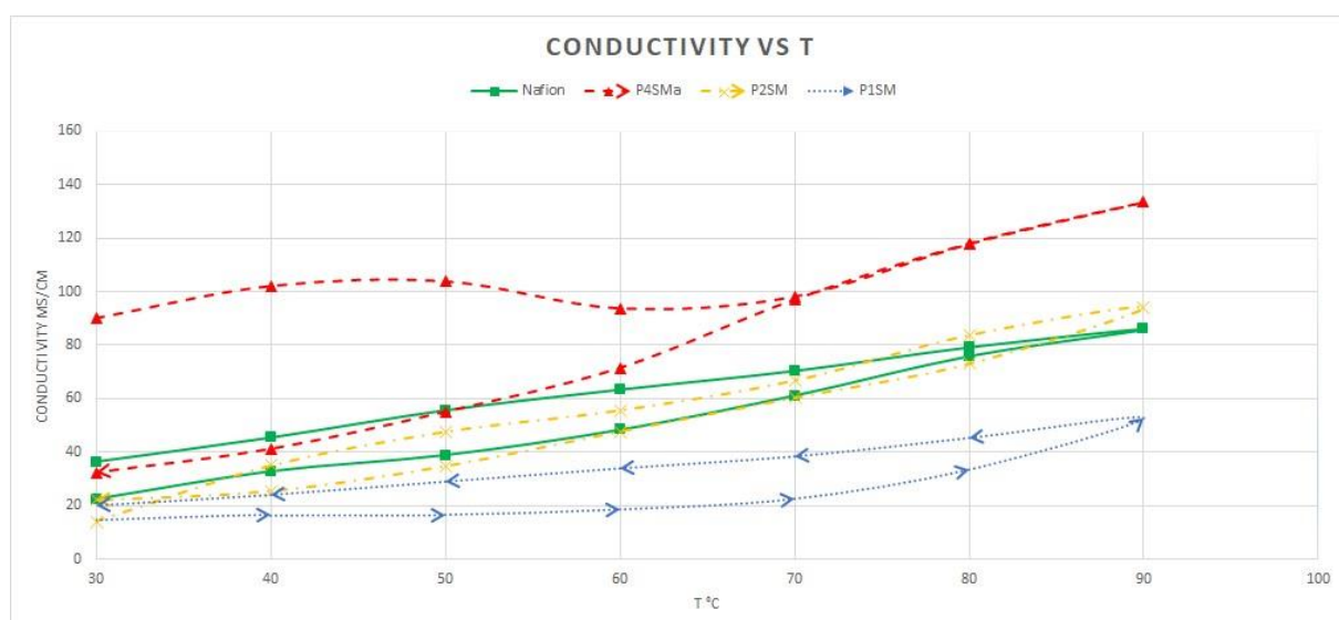
Figure IV-11. Membrane Conductivity vs. temperature.
