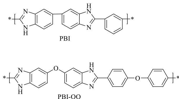
Figure IV-8. PBI and PBI-OO chemical formulas.
