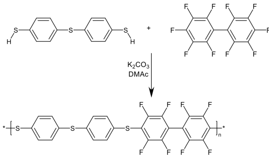
Figure II-15. Polycondensation of TBBT and decafluorobiphenyl
