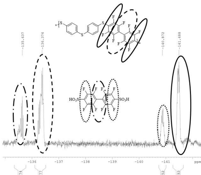
Figure III-33. 19 F NMR spectrum obtained after attempted sulfonation.
