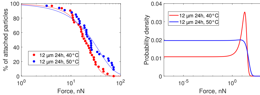
Figure 11: (left) Percentage of attached particles as a function of applied force for 12 \mu\text{m} particles dried for 24h at different drying temperatures of 40°C and 50°C. (right) Probability density functions.
