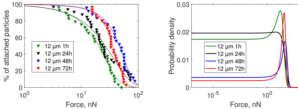
Figure 12: (left) Percentage of attached particles as a function of applied force for 12 \mu\text{m} particles dried at 50°C for 1h, 24h, 48h or 72h. (right) Probability density functions.
