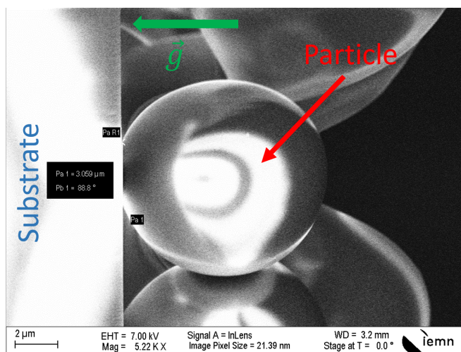
Figure 2.9: SEM image of 12 \mu\text{m} polystyrene particle in contact with the glass substrate. The contact radius is 1.53 \mu\text{m} .
