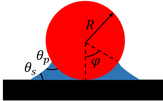
Figure 1.12: Liquid bridge formed between a particle (contact angle \theta_p ) having a radius R and a substrate (contact angle \theta_s ). The filling angle is \varphi .
