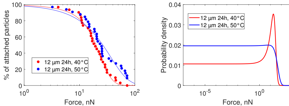
Figure I1: (left) Percentage of attached particles as a function of applied force for 12 \mu\text{m} particles dried for 24h at different drying temperatures of 40 °C and 50 °C. (right) Probability density functions.
