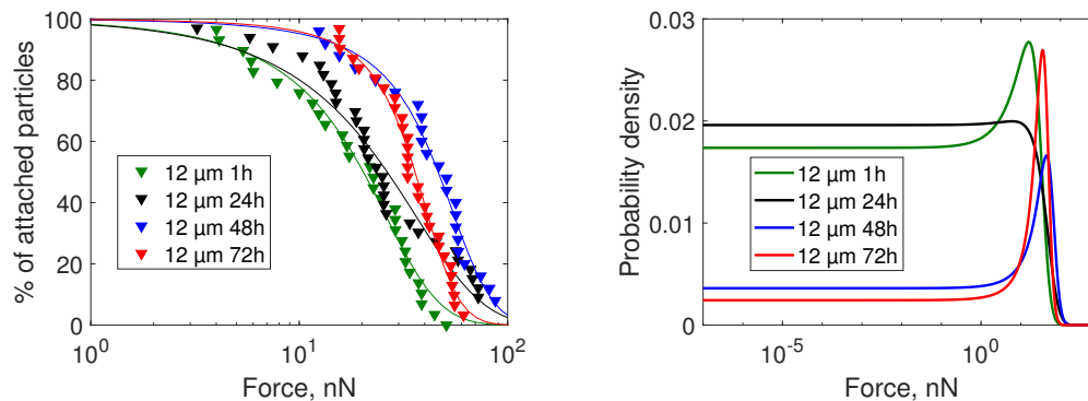
Figure I2: (left) Percentage of attached particles as a function of applied force for 12 \mu\text{m} particles dried at 50 °C for 1h, 24h, 48h or 72h. (right) Probability density functions.
