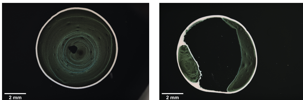
(a) Coffee-ring with uniform particle distribution inside. (b) Coffee-ring with partially uniform distribution and second contour inside.
