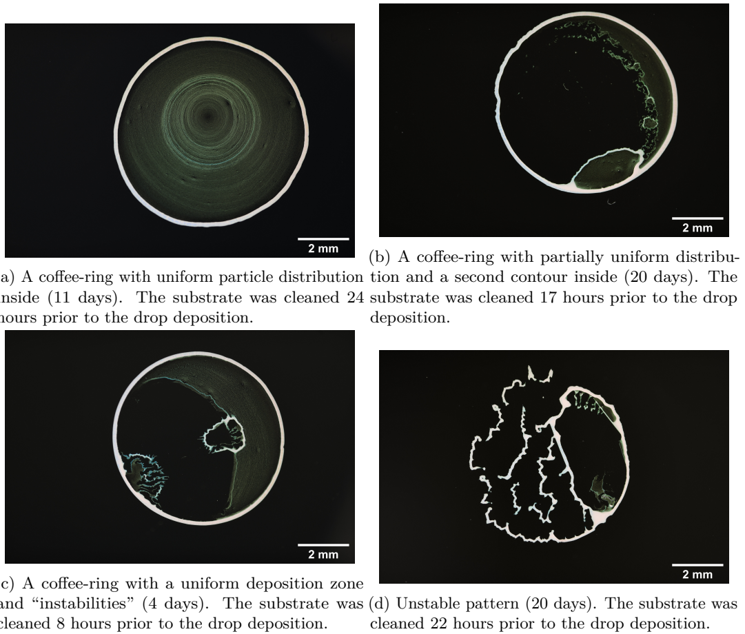
Figure 5.2: Four different patterns obtained after following our protocol. The time in brackets indicates the suspension age. The time between the substrate cleaning and the drop deposition is also given for each pattern. It will be discussed in detail in the section 5.5.1.
