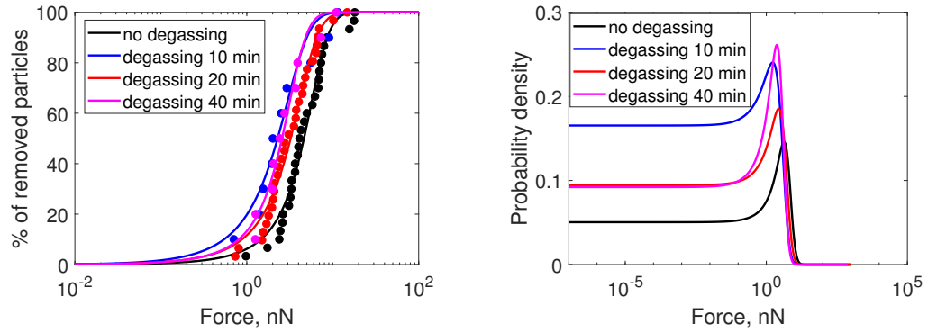
Figure II2: Hydrophobic particles placed on a hydrophilic substrate: (left) experimental curves and (right) probability density functions.
