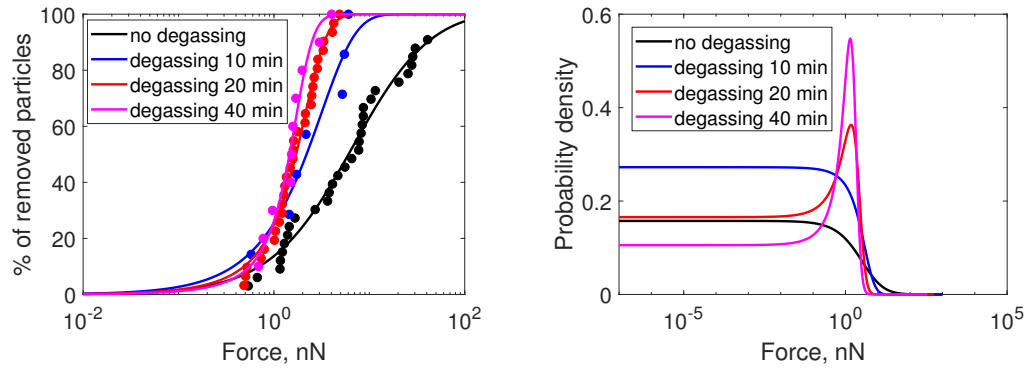
Figure II3: Hydrophilic particles placed on a hydrophobic substrate: (left) experimental curves and (right) probability density functions.
