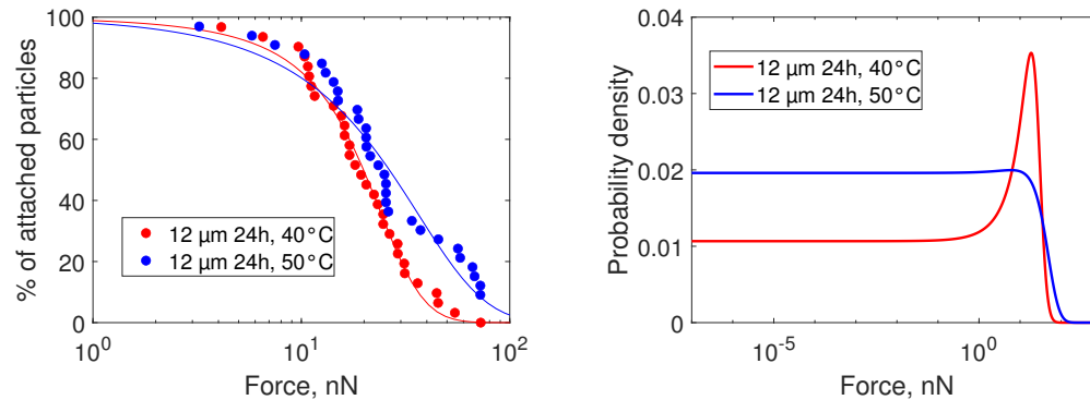
Figure 11: (left) Percentage of attached particles as a function of applied force for 12 \mu\text{m} particles dried for 24h at different drying temperatures of 40 °C and 50 °C. (right) Probability density functions.
