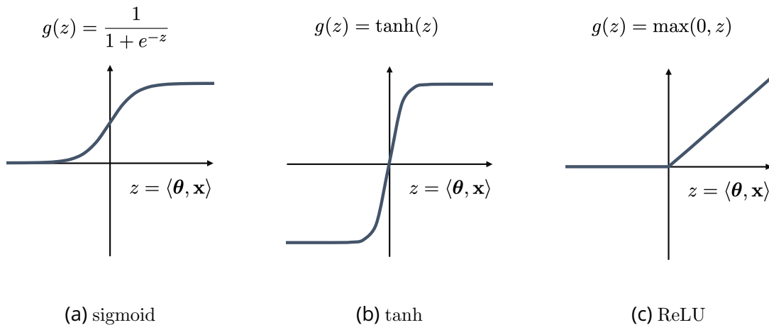
Figure 5.4: Activations functions
