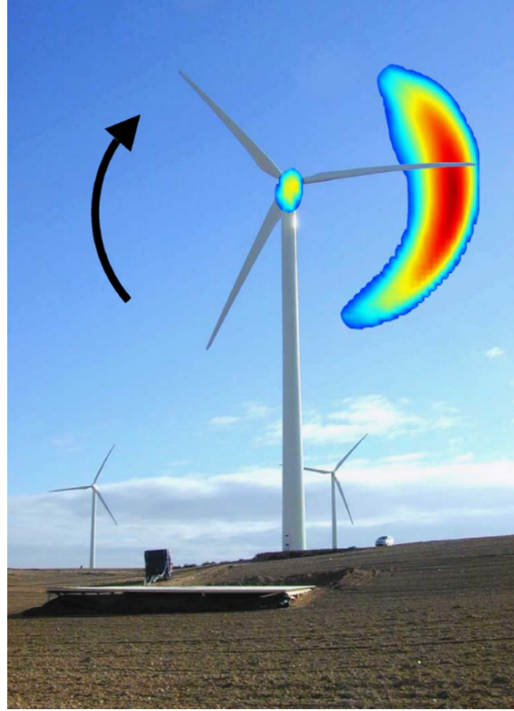
Figure 1.3: Noise source distribution in the rotor plane of a wind turbine of rotor diameter 58m, measured by Oerlemans et al. [64] with a microphone array located on a horizontal platform 58m upwind from the wind turbine.
