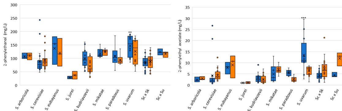
Fig. S9. Box plots of the production of aromas associated to phenylpyruvate metabolism by the different species at each temperature: ■ 16 °C and ■ 22 °C. All amounts correspond to samples taken at 60 g·L -1 of CO 2 released (~ 65% of the fermentation). Asterisks on top of a box indicate a statistically significant difference (Dunnett's multiple comparison test) with respect to S. cerevisiae . Levels of significance: p<0.05 (*), p<0.01 (**) and p<0.001 (***)
