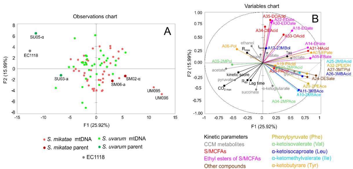
Figure 4. Principal component analysis (PCA) representing all kinetic variables and all metabolites quantified at 80 g/L of CO 2 released.
