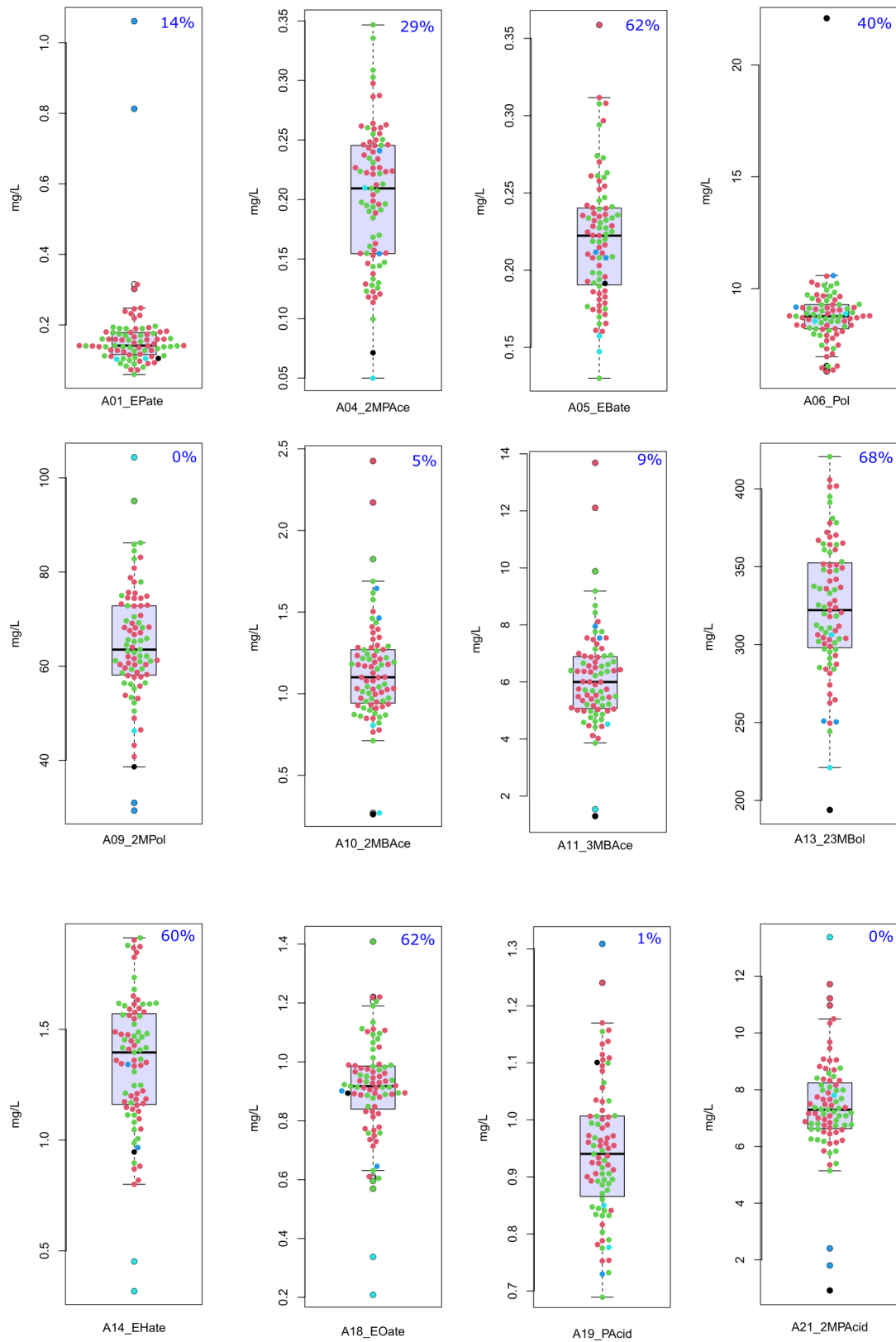
Figure S7. Boxplots showing the distribution of fermentative aromas at 80 g/L CO 2 released. The blue percentage indicates the proportion of segregants showing a transgressive phenotype.
