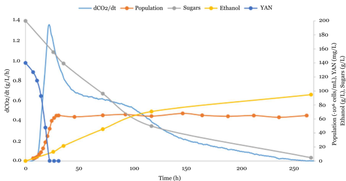
Figure 11. Evolution of the main parameters during alcoholic fermentation at 24 °C using the S. cerevisiae Lalvin EC1118® in synthetic must.
