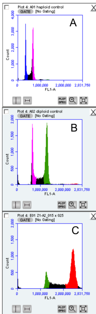
Figure S3. Example of ploidy estimation using flow cytometry. A: haploid S. cerevisiae control. B: diploid S. cerevisiae control. C: hybrid T2o.
