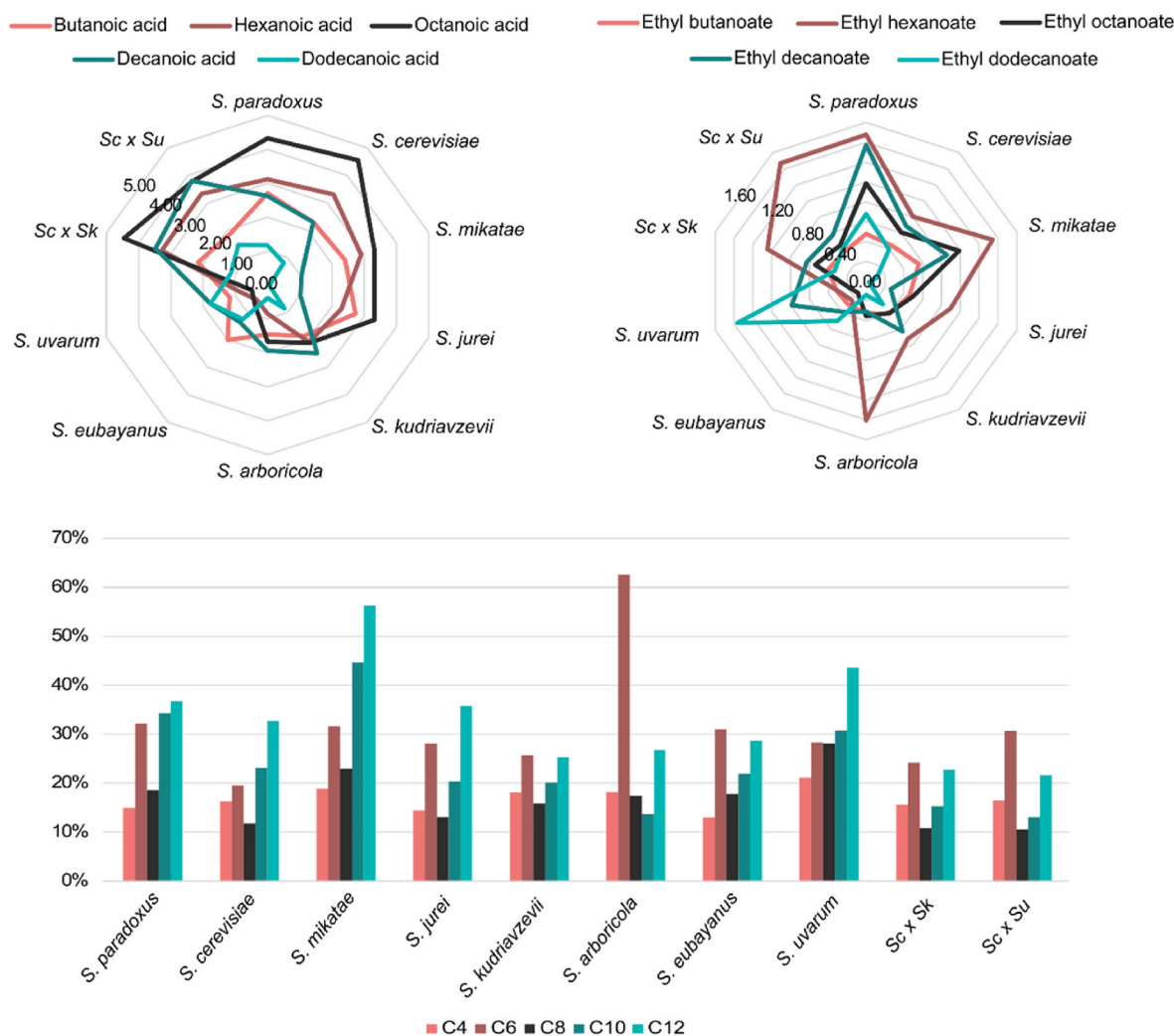
Fig. 8. Representation of the amounts of S/MCFAs (A) and their ethyl esters (B) secreted into the medium by each species, shown as the equivalent in CoA used for the production of each molecule, in mmol·L -1 . CoA equivalents were calculated from the concentration of a given compound, by dividing with the number of acetyl-CoA molecules used for its production (i.e. the number of carbon atoms in its chain divided by two). Subfigure C shows the proportion of each ester relative to its fatty acid counterpart, for each chain length (C4 – C12). All graphs correspond to fermentations at 22 °C.
