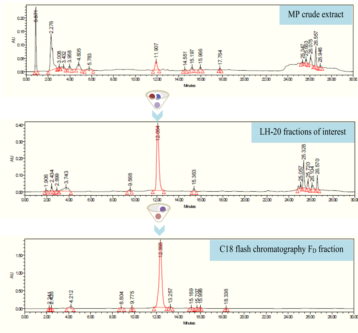
Figure 23: HPLC-UV chromatograms at 254nm depicting the qualitative profiles of the crude extract (top), the fraction of interest after a fractionation through a LH-20 column (middle) and a purification through a C18 column thereof (bottom). The height of the Y-axes is not representative of the compound proportion retrieved from the crude extract. C18 (150 x 4.6 mm, 3µm). A: H 2 O and B: MeOH/ H 2 O 50/50. Flow 0.7 mL/min.
