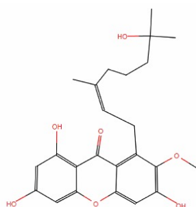
hypothesis m
