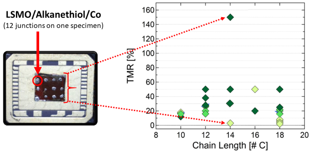
Figure 1.14: TMR measurements on LSMO/Alkanethiol/Co systems from C10, C12, C14, C16 and C18 (in the right), different TMR amplitudes have been detected from one specimen containing 12 junctions (in the left), figure is adapted from [26].
