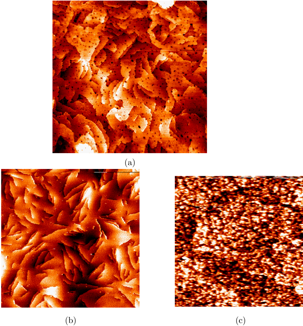
Figure 3.11: STM images, (a) Fe(001)/MgO(001) no ex situ cleaning, , STM 400 \times 1 = 400nm^2 image of Iron surface ( I_T = 0.36nA , U_{gap} = -0.218V ), color scale: \Delta z = 0.5nm , (b) Fe(001)/MgO(001) after UV/ozone surface cleaning of MgO substrate, STM 400 \times 400nm^2 image of Iron surface ( I_T = 0.012nA , U_{gap} = 0.822V ), color scale: \Delta z = 0.4nm , edges of the image are aligned with Fe[100], (c) C16MT/Fe(001)/MgO(001) , 75 \times 75nm^2 ( I_T = 15pA , U_{gap} = -1.9V ) surface image of C16MT grafted on Fe(001).
