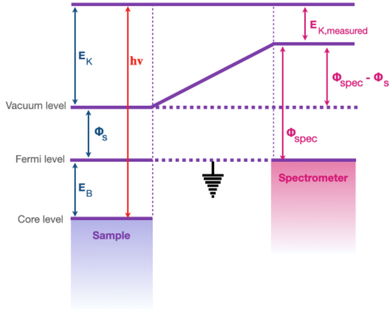
Figure 2.2: Scheme of the energy configuration taking place in a photoemission experiment where the spectrometer is electrically connected to the solid sample.
