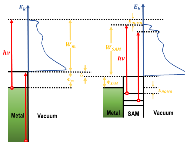
Figure 3.13: Energy relationships in UPS, left for metal system, and right for an organic layer deposited on the metal substrate. \Delta :vacuum shift (presence of a dipole moment at the interface), E_{HOMO} : energy of the highest occupied molecular orbital
