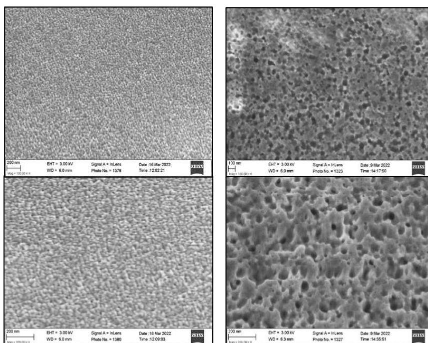
Figure 2-36 SEM images of a) flat TiN, b) 6-minute etched TiN at 100 KX (top) and 200 KX (bottom) magnification.
