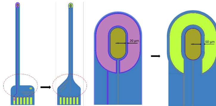
Figure 2-18 Improvement in geometric structure of model 3-b.
