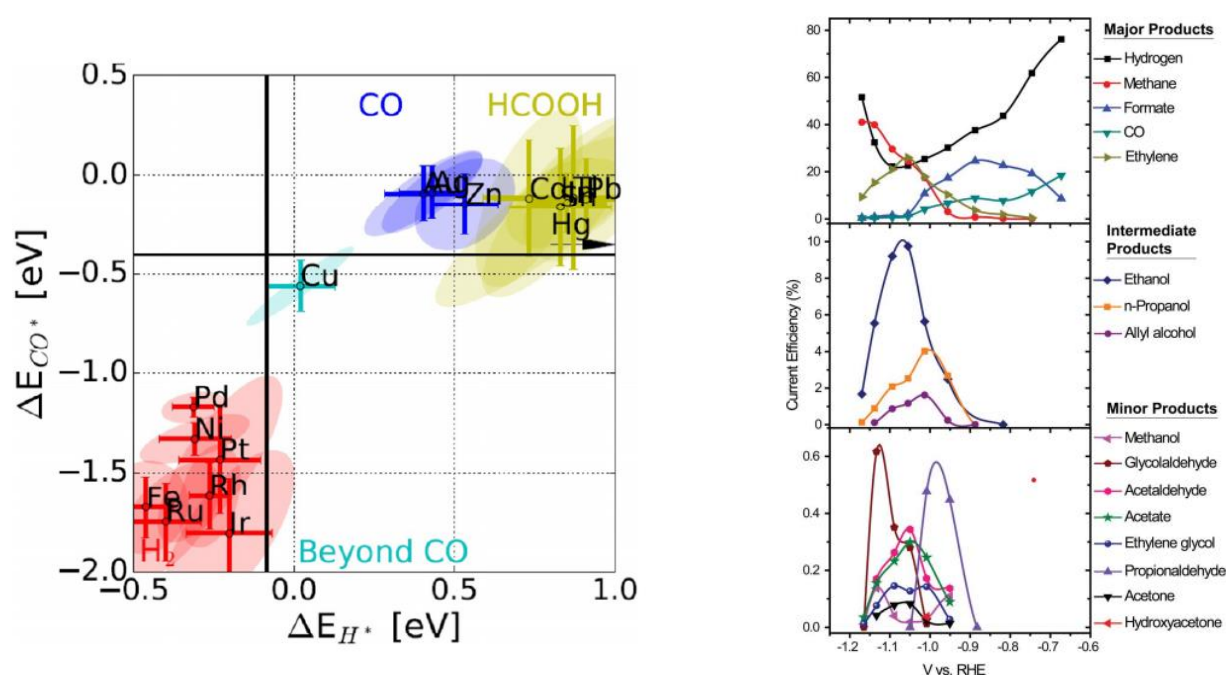
Figure 1-3. Binding energies of the intermediates ( H^* and CO^* ) for different metal catalysts (left). Reproduced from Bagger et al. 22 . Current efficiency in function of potential for each reaction product of a copper catalyst. Reproduced from Jaramillo et al. 33 .
