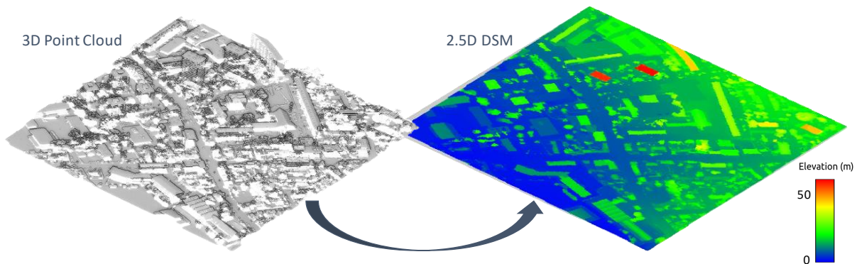
Figure 8: Illustration of a 3D point cloud and its corresponding rasterization into 2.5D DSM. The DSM is colored as function of the height.
