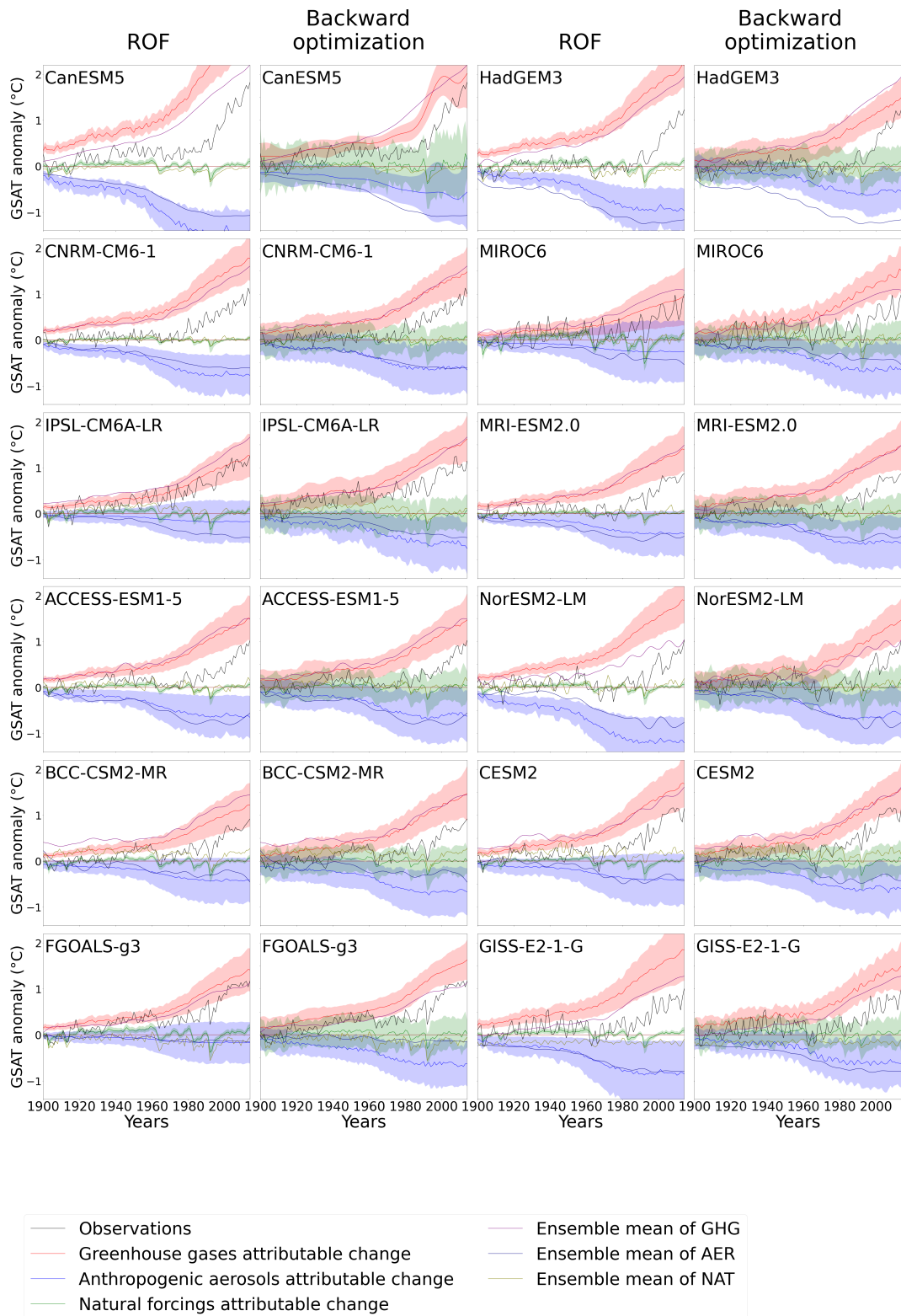
Figure 7. Attributable GSAT in °C calculated for ROF and backward optimization from (black line) a HIST member. The GSAT is decomposed into the attributable changes due to (red line) greenhouse gases; (blue line) anthropogenic aerosols and (green line) natural forcings. For comparison, the ensemble mean of (purple line) GHG, (dark blue line) AER and (beige line) NAT is indicated. Color shades show the 90% confidence intervals of the attributed GSAT.
