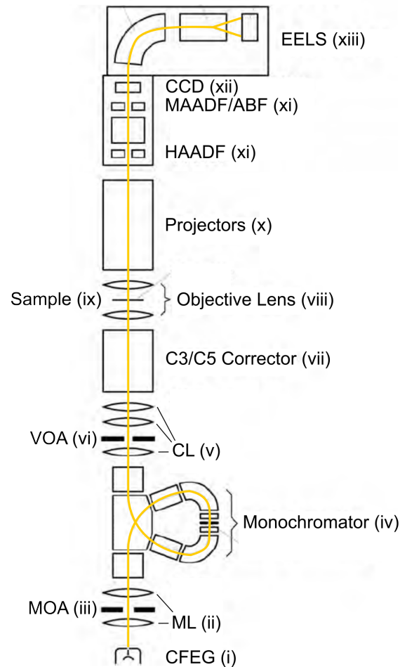
Figure 2.1: Schematic cross-section of Nion UltraSTEM TM with a monochromator. The electron beam travels from bottom to top, marked in yellow. Reproduced from ref. [23].
