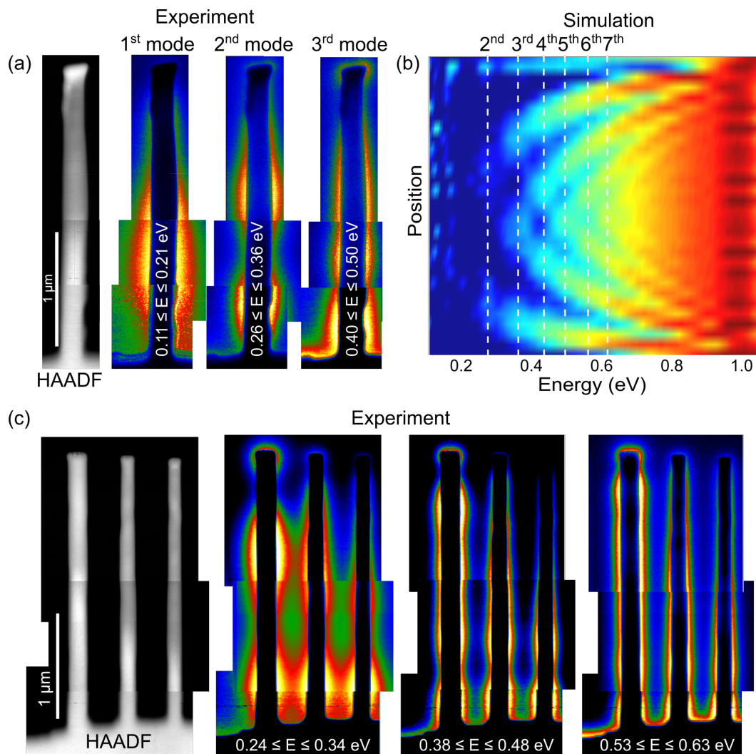
Figure 3.12: (a) HAADF image and the energy-filtered STEM-EELS maps and (b) two-dimensional simulated EELS map of the 2.5 \mu\text{m} length half-rod. The white dashed lines highlight the energy of simulated LSP modes. (c) HAADF image and the energy-filtered STEM-EELS maps of the 2.5 \mu\text{m} length triple neighboring half-rods.
