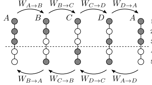
Figure 7.2: Loop of four configurations with N = 3 agents on M = 5 sites breaking Kolmogorov's criterion when the utility is non-linear and is a function of an individual perceived density. Shaded and unshaded nodes correspond to occupied and empty sites respectively. The dashed line indicates a possible segmentation of the system into two distinct neighborhoods.
