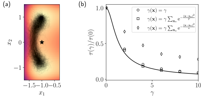
Figure 8.3: (a) Sample of trajectories going from one well to another in almost directly (here leaving \mathbf{x}(0) = [-1 \ 1]^T and reaching a small circle around \mathbf{x} = [-1 \ -1]^T ) for the complicated force field illustrated in Fig. 8.2(b), albeit for T = 0.3 . The black star represents the saddle point of the original potential, which is clearly not visited by the most probable trajectories in the modified force field. (b) Comparison of the reduction in relaxation time (measured by fitting the relaxation dynamics of the position) for the original IO forcing and the two force fields of Fig. 8.2 ( T = 0.1 ). The continuous line represents the full Eyring-Kramers prediction of the standard IO acceleration.
