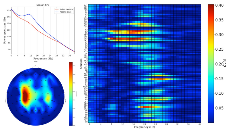
Figure 3.12: Needed representation to evaluate subjects' performance: Top Left: visualization of the average spectral estimation (Burg estimator in this case) for motor imagery (in red) and resting state (in blue) for a specific electrode. Bottom Left: Topography map for a certain frequency bin, colormap corresponds to the level of significant differences between the two cognitive states. Right: Statistical difference map (here coefficient of determination) for each electrode for each frequency bin computed over trials of the different cognitive states.
