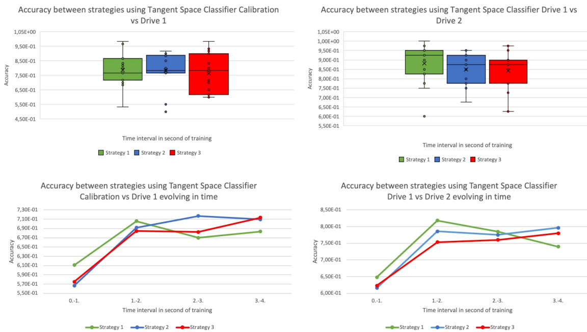
Figure E.1: Top: Accuracy in the different phases using the tangent space logistic regression on the covariance matrix computed on the time series of motor imagery and resting state. Bottom: Average accuracy for the different strategies with training on the different intervals of time to assess the evolution of the accuracy with regards to the interval.
