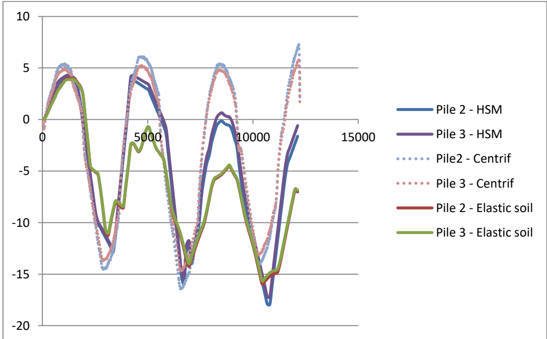
Figure V. 22 - Comparison of head load variations between experimental results, an elastic soil model and an HSM model for Pile 2 and Pile 3
