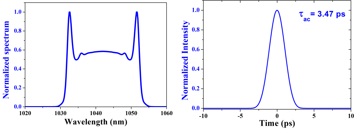
Figure 4.5: (Left) Simulated spectrum obtained at the output of ANDi laser. The spectral width is \sim 22 nm, while the spectrum has a characteristic shape of ‘cat-ear’ or ‘Batman’. (Right) The corresponding autocorrelation trace with \tau_{ac} \sim 3.47 ps.
