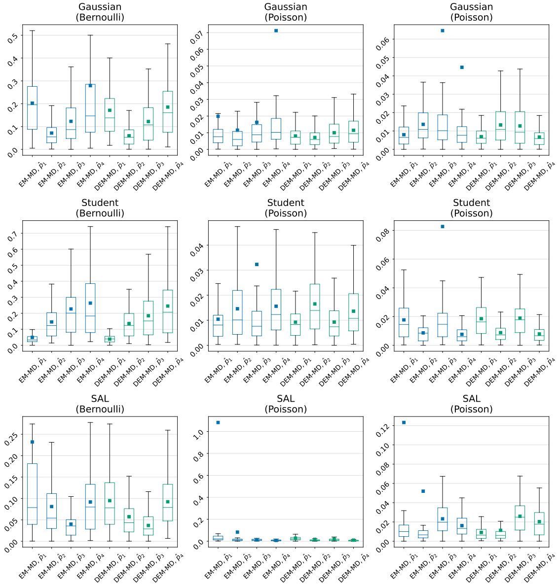
Figure 4.10: Boxplots of relative discrete distribution parameter errors for settings C_{524} (a), C_{423} (b) and C_{223}^P (c) on both DEM-MD (green) and EM-MD (blue). In each subplot, a row corresponds to a continuous distribution (Gaussian, Student, SAL in this order).
