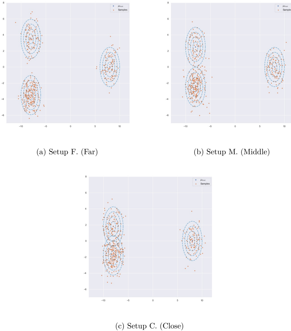
Figure 3.4: Gaussian mixture distributions for Setups F., M. and C. involved in Cases presented in Table 3.A.3.2 with an example of sampled data sets. Blue crosses correspond to \mu_k and ellipses to covariance matrices \Sigma_k . Orange points are samples.
