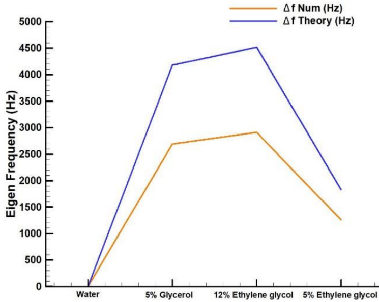
Figure 2.17: Theoretical and numerical shifts eigen frequency were calculated according to[32] at mode 13th.
