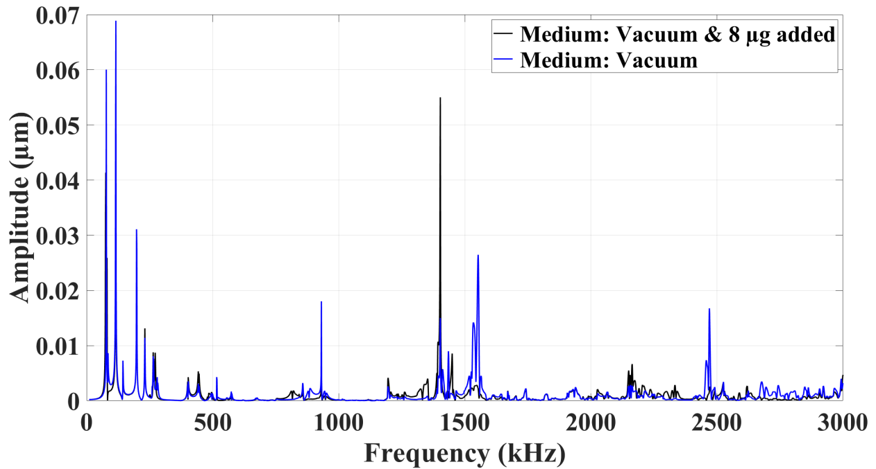
Figure 4.32: Amplitude response in vacuum (blue), and with 8 \mu g added to the beams (black).
